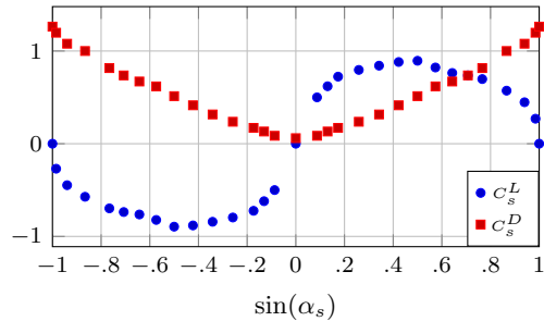
(a) Value of C_s^L and C_s^D v.s. sinus of the attack angle \alpha_s (from [19, p. 86]).
