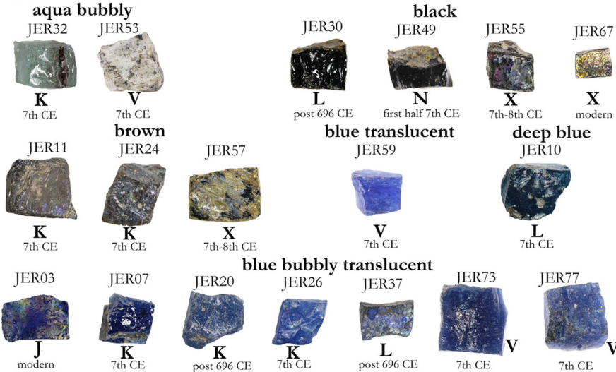
Figures 2 and 3 Specimens from the North Western Quarter divided by base glass composition and colour, with an indication of sample number, trench letter and date of the backfill.
