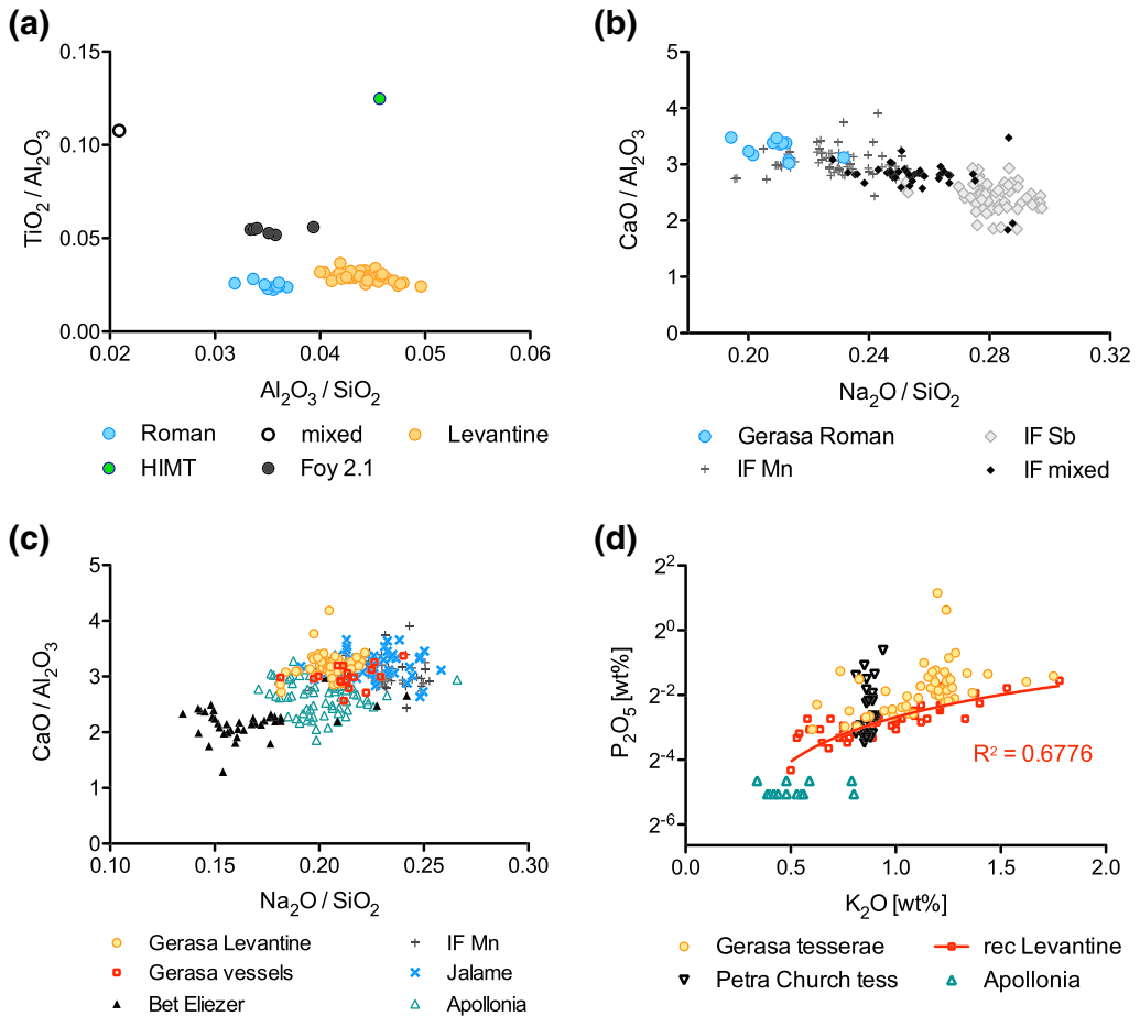
Figure 4 Base glass characteristics of the Gerasa tesserae divided by compositional groups. (a) The ratios of Al_2O_3/SiO_2 and TiO_2/Al_2O_3 reflect the feldspar and heavy mineral composition of the silica sources and separate the different base glass groups. (b) The Na_2O/SiO_2 and CaO/Al_2O_3 ratios of the Roman tesserae from Gerasa compared with different Roman glass reference groups (Roman Sb, Roman Mn, Roman mixed) based on the glass finds from the Iulia Felix shipwreck (IF). (c) Comparison of the Na_2O/SiO_2 and CaO/Al_2O_3 ratios of the Levantine I tesserae and vessels from Gerasa with primary production groups from the Levantine coast, including Mn glass from the Iulia Felix shipwreck (IF Mn) and glass from Apollonia, Bet Eliezer and Jalame. (d) The K_2O and P_2O_5 concentrations of the Gerasa tesserae compared with glass from the primary furnace at Apollonia, recycled Levantine glasses from Jordan and tesserae from the Petra Church in Jordan (y-axis in \log_2 ). Sources: Iulia Felix shipwreck (Silvestri 2008; Silvestri et al. 2008); Jalame (Brill 1999); Apollonia (Brens et al. 2018; Freestone et al. 2008; Phelps et al. 2016); Bet Eliezer (Freestone et al. 2000); Levantine vessels glass from Gerasa (Barford et al. 2018) and Umm el-Jimal (Al-Bashaireh et al. 2016a), window panes (Schibille et al. 2008) and Petra Church tesserae (Marii and Rehren 2009).
