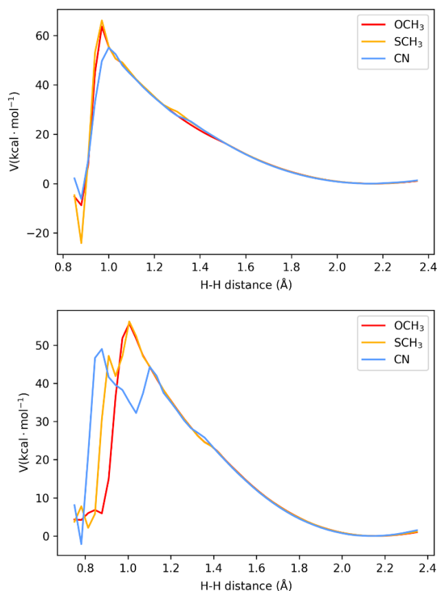
Figure 5: Potential energy surface for H-H distances for the two-proton, two-electron (top) and three-proton, two electron (bottom) mechanisms. The three-proton mechanism shows the presence of high-energy intermediates for two of the complexes, associated with one proton between TFA - and the bound second proton. See Figures S4-S6 for representations of the highest energy states.
