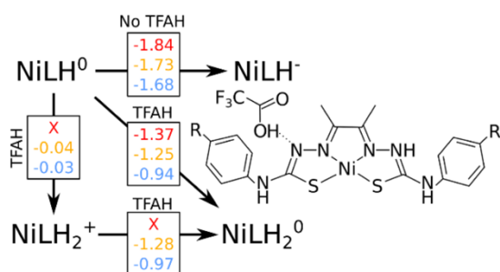
Figure 4: Free energy diagram considering the second protonation to the second N d atom. Red, yellow and blue numbers are free energy differences corresponding to OCH 3 , SCH 3 and CN substituents, respectively. The NiOCH 3 complex is spontaneously protonated in the presence of TFAH. All numbers are in eV.
