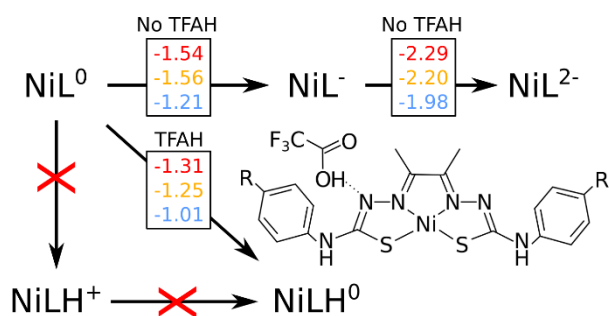
Figure 2: Free energy diagram considering the first protonation, as well as first and second reduction steps. Red, yellow and blue numbers are free energy differences corresponding to \text{OCH}_3 , \text{SCH}_3 and \text{CN} substituents, respectively. All number are in eV.
