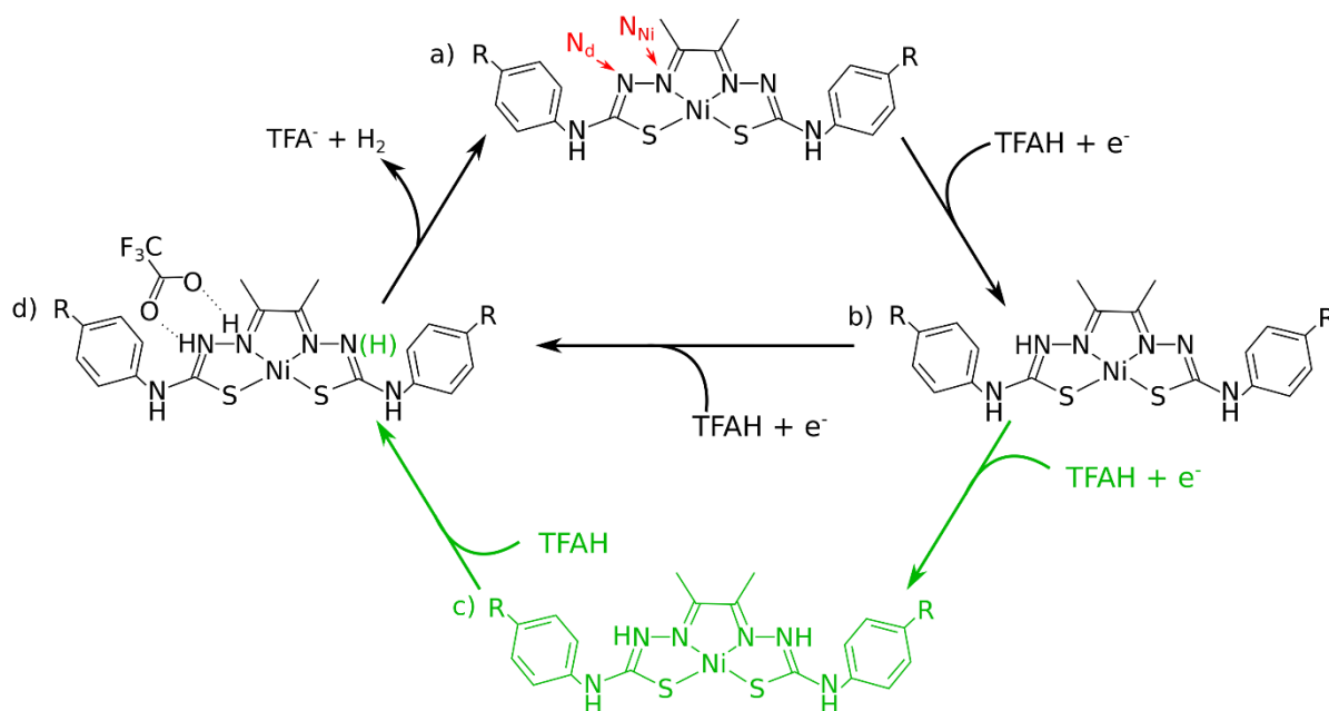
Figure 1: The two-proton, two-electron proposed catalytic cycle for the series of NiL complexes investigated in this study. R = OCH 3 , SCH 3 and CN. In red, we indicate the notation adopted for this article, where N Ni corresponds to the coordinating N atoms, and N d is the distal N atom further away from Ni. TFA - and TFAH corresponds to the anionic conjugated base and the neutral protonated form of TFA, respectively. Protonation sites were determined based on calculated relative pK a values. A possibility of a three-proton scenario is also considered (in green), with both N d protonated prior to protonation of one of the N Ni atoms.
