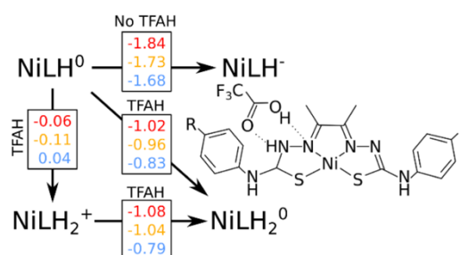
Figure 3: Free energy diagram considering the second protonation to two adjacent N atoms ( \text{N}_d and \text{N}_{Ni} ) and the final step of the cycle. Red, yellow and blue numbers are free energy differences corresponding to \text{OCH}_3 , \text{SCH}_3 and \text{CN} substituents, respectively. All number are in eV.
