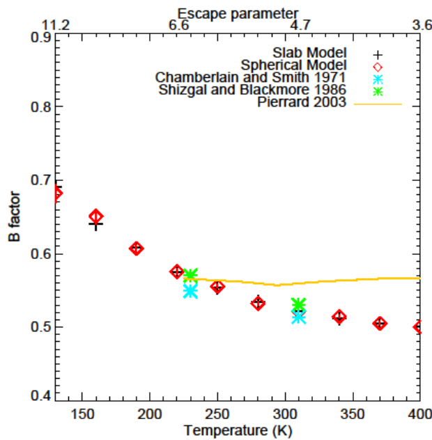
346 347 Fig. 3: Simulated B factor for Mars for the slab isothermal model (black) and the spherical isothermal model (red) at 348 different atmospheric temperatures. The results from other studies (slab models): Chamberlain and Smith (1971) and 349 Shizgal and Blackmore (1986); spherical (Pierrard 2003) are also displayed for comparisons.
