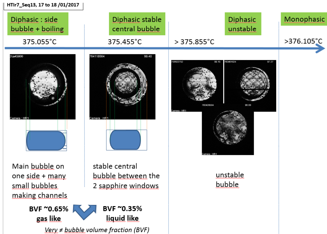
Fig. 2 : Some experimental observations on the gas and liquid partitioning as a function of temperature in microgravity for the SCWM case
