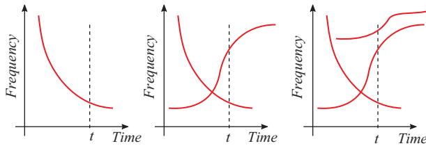
Figure 2.1 Evolution of the IF for both mono-component and multicomponent signals
