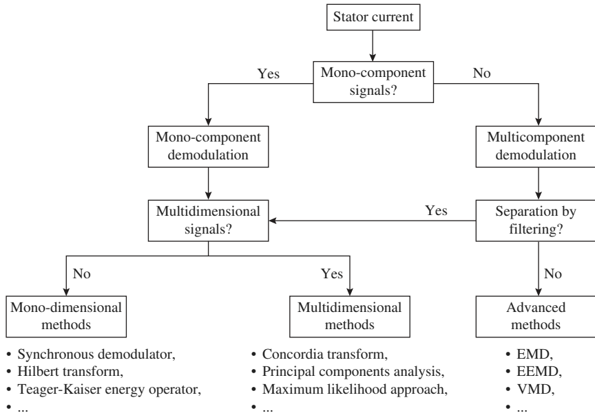
Figure 2.2 Road map to choose the demodulation technique
