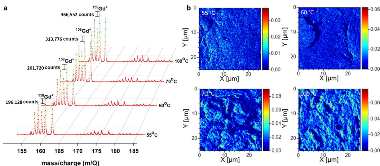
Figure 5. (a) ToF-SIMS spectra shows increased Gd counts for samples with a higher degree of functionalization (due to the increased reaction temperature). (b) ToF-SIMS element distribution maps reveals the evenly distribution of Gd complex on the carbon nanotube (CNT) surface and further increment of Gd percentage in the CNTs with respect to increased reaction temperature can also be visualized (bright contrast increment).
