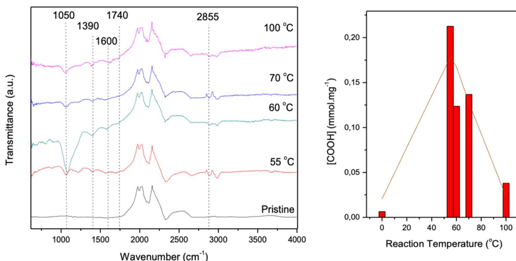
Figure S1: CNT Functionalisation analysis: a) FT-IR spectra of MWNTs treated at varied oxidative temperatures showing characteristic -COOH peak at \sim 1700 cm -1 wavenumber . b) Boehm Titration results of carboxylic groups present on acid treated carbon nanotubes with varied temperature conditions.
