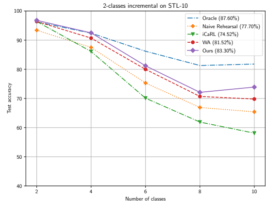
Fig. 3. Comparison of different rehearsal strategies initialized with a self-supervised encoder. Legend gives the average accuracy for each method.
