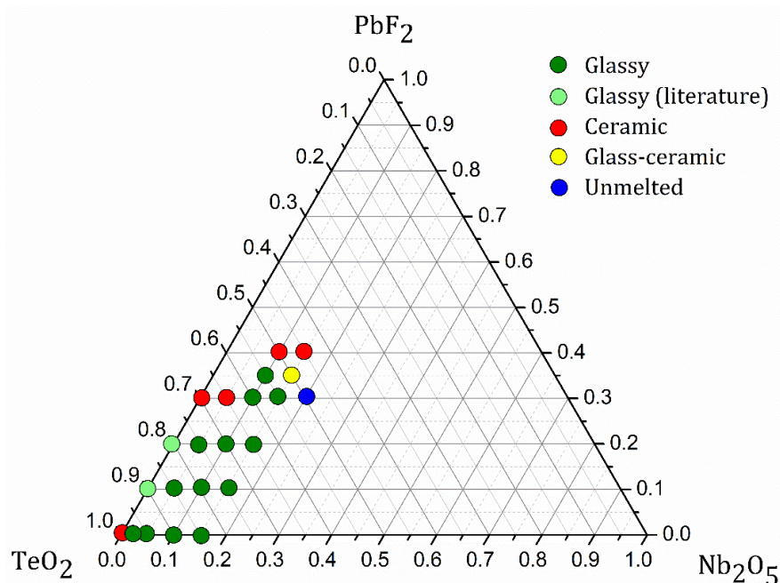
Figure 1. Glass-forming domain in the ternary system \text{TeO}_2 - \text{Nb}_2\text{O}_5 - \text{PbF}_2 .
