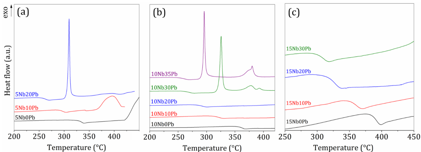
Figure 2. DSC curves of glasses in the glass series (a) 5Nb by Pb, (b) 10Nb by Pb and (c) 15Nb by Pb.
