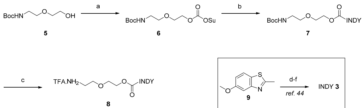
Scheme 2. Preparation of INDY 3 and fragment 8 . Reagents and conditions: (a) DSC (2.0 equiv), \text{NEt}_3 (2.0 equiv), ACN, rt, 2 h (quant.); (b) 3 (1.0 equiv), NaH (1.1 equiv) then 6 (1.1 equiv), DMF, rt, 0.5 h (75%); (c) TFA excess, DCM, rt, 0.5 h (quant.); (d) Ethyl iodide (15 equiv), sealed tube, 80 °C, 5 days (96%); (e) \text{Ac}_2\text{O} (2.3 equiv), \text{NEt}_3 (2.4 equiv), ACN, reflux, 3 h (84%); (f) \text{BBr}_3 (2.0 equiv), DCM, 0 °C to rt, 24 h (95%).
