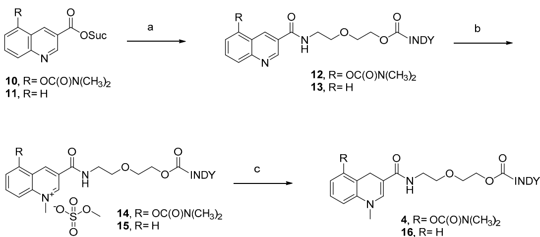
Scheme 3. Grafting of fragment 8 to quinoline moieties. Reagents and conditions: (a) 8 (1.0 equiv), \text{NEt}_3 (5.0 equiv), ACN, 0 °C to rt, 0.5 h ( 12 : 71%, 13 : 98%); (b) \text{Me}_2\text{SO}_4 (1.1 equiv), DCE, sealed tube, 50 °C, 24 h ( 14 : 93%, 15 : 86%); (c) BNAH (1.0 equiv), DCM, rt, 0.5 h ( 4 : 72%, 16 : 80%).
