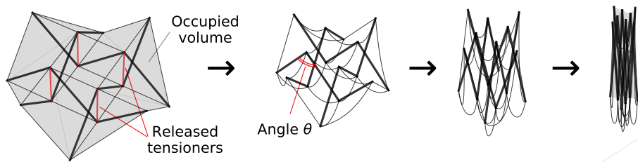
Figure 5: Folding process of a “Tensarch” module 3×3.
