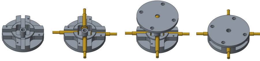
Figure 22: Connection to layer cables.
