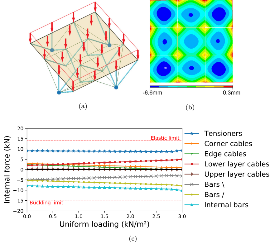
Figure 11: (a) Illustration of a 3 \times 3 module on 4 edge supports under uniform load case. (b) Vertical displacements maps of the deck plates under a loading of 3 \text{ kN/m}^2 . (c) Variation of internal forces in a 3 \times 3 module as the load increases incrementally.
