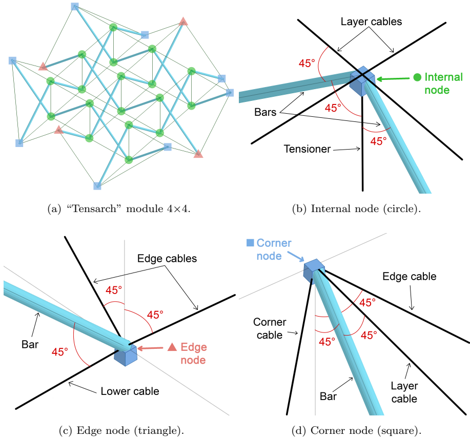
Figure 19: Different types of nodes of a “Tensarch” module 4×4.
