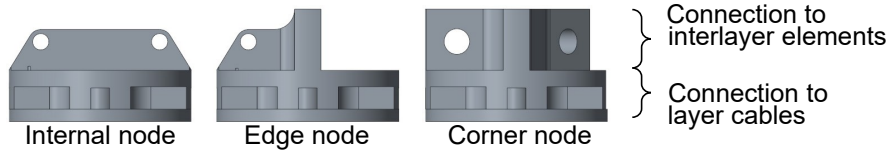
Figure 20: Body parts for the 3 categories of nodes.
