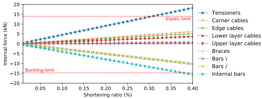
Figure 10: Evolution of internal forces in function of shortening ratio of the tensioners.
