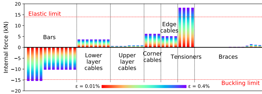
Figure 9: Spectrum of internal forces in the elements in function of self-stress state.
