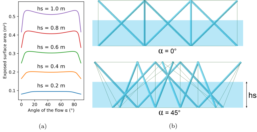
Figure 16: (a) Exposed surface area of a module 3 \times 3 for different submerged heights h_s . (b) Illustrations of a submerged module 3 \times 3 viewed from different angles.
