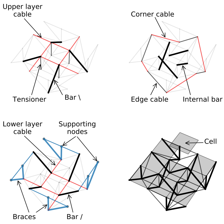
Figure 7: Composition of a single platform module 3x3.
