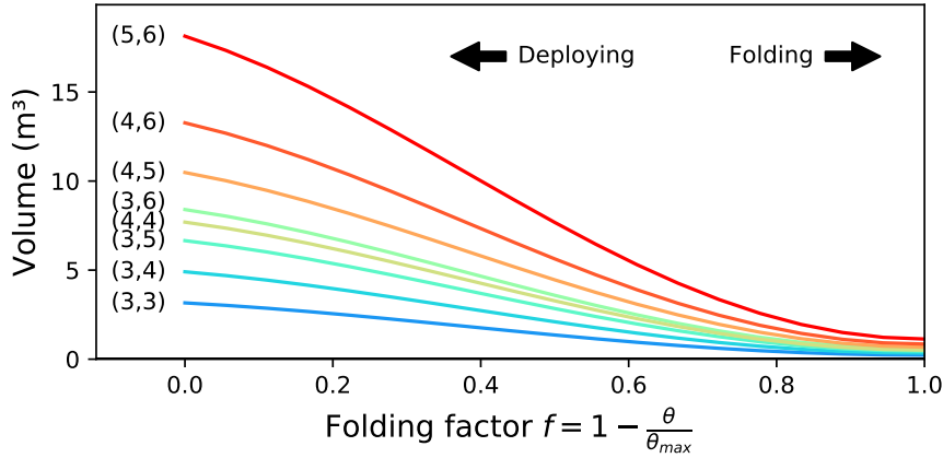
Figure 6: Volume occupied by “Tensarch” modules during folding and deployment process for a cell size of 1 \text{ m}^3 .
