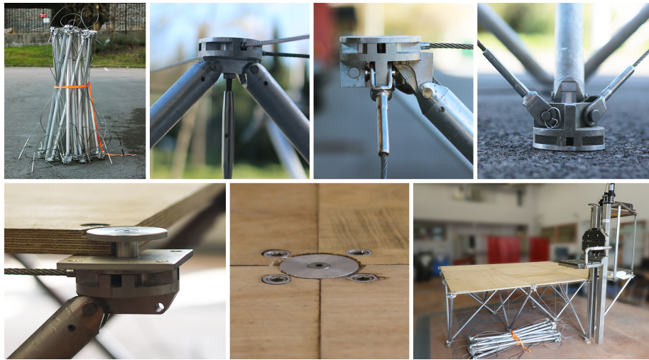
Figure 26: Assembly of the prototype's components.
