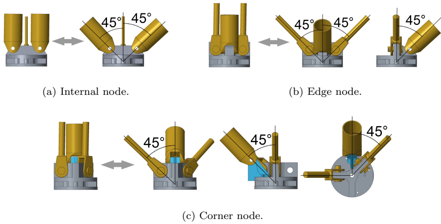
Figure 23: Visualization of incidence angles of the connected interlayer elements and their folding mechanisms at each node of the structure.
