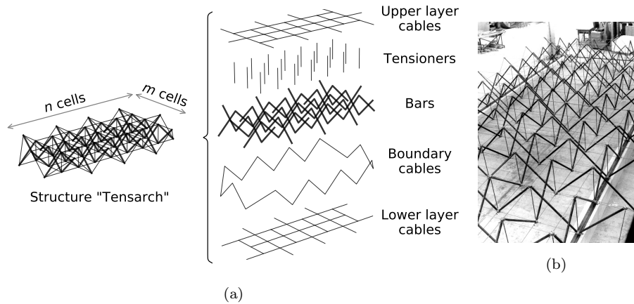
Figure 4: (a) Elements composing the “Tensarch” structure. (b) “Tensarch” 80 m 2 prototype.
