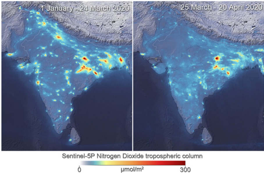
Fig. 6 Nitrogen dioxide levels before (left) and during the lockdown in India in 2020. \text{NO}_2 mean levels decreased by about 40–50% from the January 1–March 24 periods to the March 25–April 20 period. Noteworthy, high \text{NO}_2 concentrations coincide with the location of power plants. Modified from Copernicus Sentinel data (2019–20), processed by ESA, CC BY-SA 3.0 IGO (ESA 2020c)
