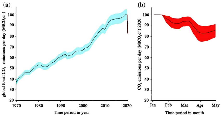
Fig. 7 Fossil fuel \text{CO}_2 emissions ( \text{MtCO}_2 \text{d}^{-1} ) for the 1970–2019 timeline compared to during the COVID-19 confinement period (2020). Blue shading showing annual \text{CO}_2 emissions from 1970 to 2019 (a). \text{CO}_2 emissions have been nearly upward trend every year, with about 100 \text{ MtCO}_2 \text{d}^{-1} being released in late 2019. Conversely, since early 2020, red shading shows a significant decrease in carbon emissions during confinement (b). On April 7, 2020, the influence of the confinement on daily global \text{CO}_2 emissions was around -17 \text{ MtCO}_2 \text{d}^{-1} ( -17\% ) in contrast to the average level of emissions in 2019. Also, during January–April 2020, \text{CO}_2 emissions fell by 1.048 \text{ MtCO}_2 \text{d}^{-1} ( 8.6\% ) compared to 2019 levels. Modified after Le Quééré et al. (2020)
