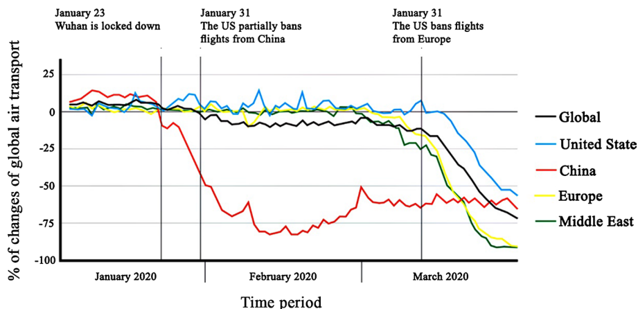
Fig. 11 Comparison of airline travel in 2020 for the COVID-19 period to the same time period in 2019. The global aviation industry slash flights as COVID-19 hits travel demand. In the context of the COVID-19 episode, strict lockdown laws have been enacted in some cities around the world. On January 23, 2020, the lockdown was implemented in Wuhan, which, as it turns out significantly reduced air travel up to -75\% —the biggest reduction to date by a China—in mid-February 2020. As of January 31, 2020, the United States imposed strict rules such as a flight ban from Europe and China, which did not see significant changes, but about two months later (late March) drastically reduce about -50\% was likely due to the US government's lockdown has been observed. Modified after Wastnage (2020)
