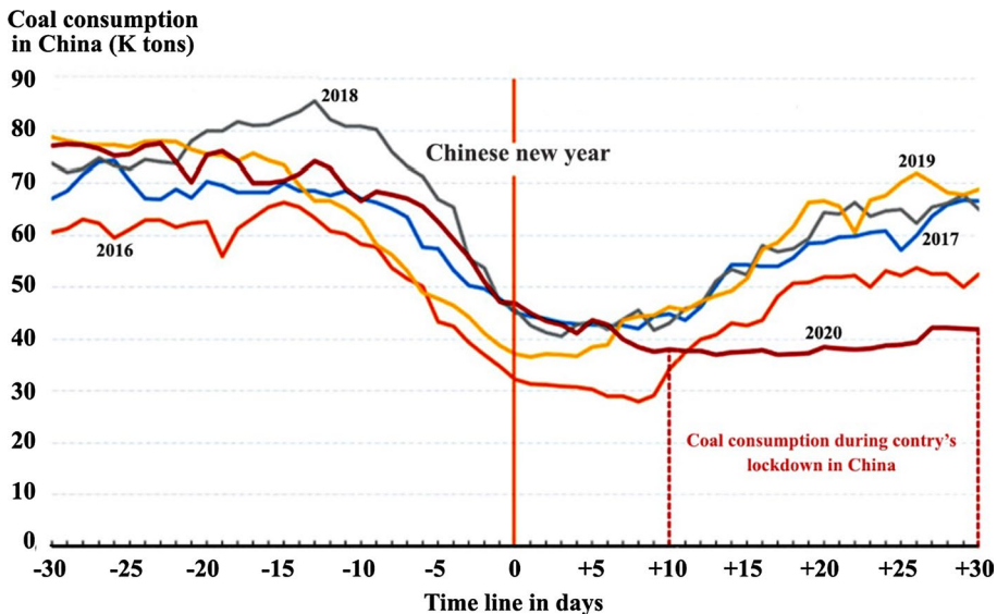
Fig. 2 Use of coal fuel in China in 2016–2020. The consumption drop for all years during the Chinese new year is explained by holidays with industrial shutdowns. In 2020 coal consumption is drastically reduced to 40 K tons during the lockdown, 10–30 days after the new year, versus about 80 K tons before the COVID episode (Ghosh 2020)
