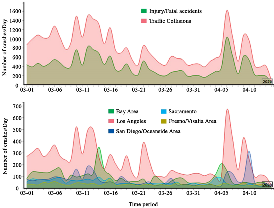
Fig. 9 California crashes during “Shelter-in-Place” orders, when heavy rains in Southern California brought a brief return to “normal” conditions: (top) the number per day of all crashes and the number of collisions/day where an injury/fatality happened, (bottom) the rates of crashes occurred between March and April 2020. Both graphs show a significant reduction in collisions particularly following heavy rains, implying the positive impact of the pandemic. Modified after Shilling and Waetjen (2020)
