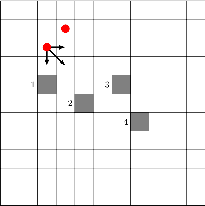
Figure A.1: Search of a lost object in the sea
