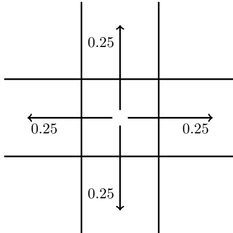
Figure 1: Transition probabilities
