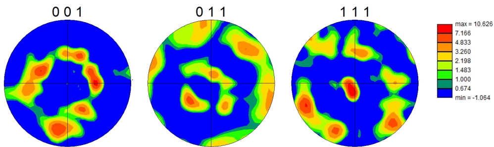
(c) ACCA 1 mm 400°C - 6h - copper
