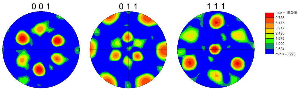
(a) ACCA 3 mm 400°C - 6h - copper
