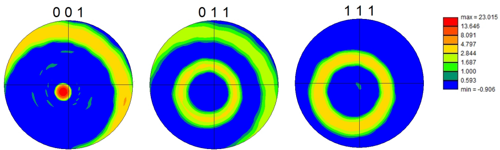
(b) ACCA 3 mm 400°C - 6h - aluminum
