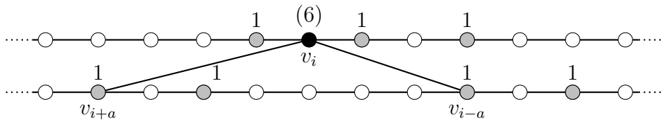
(b) Item 1: f(v_i) = 6 , a = 8 and r = 7 (so that p = 2 and n = 23 )
