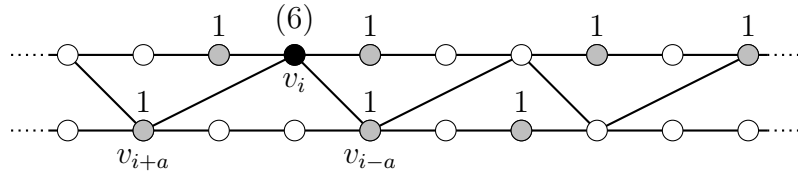
(d) Item 3: f(v_i) = 6 , a = 12 and r = 3 (so that d = 2 and n = 27 )
