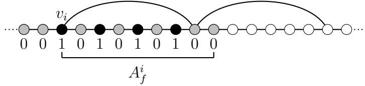
The vertices of the set A_f^i , a = 7
