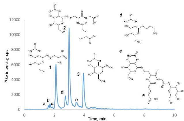
Fig. 3 Speciation of low-molecular weight (cutoff 3 kDa) water-soluble selenium in liver from turkey fed high Se (5 µg Se/g). Shown as a representative RP HPLC – ICP MS chromatogram. The Se species were identified by electrospray MS in a parallel experiment. 1, m/z 405; 2, m/z 591; 3, m/z 300. Minor selenospecies: a, b, c, not identified; d, m/z 361 (cysteinyl-SeGalNac); e, m/z 753 (glutathionyl-hexose-SeGalNac).
