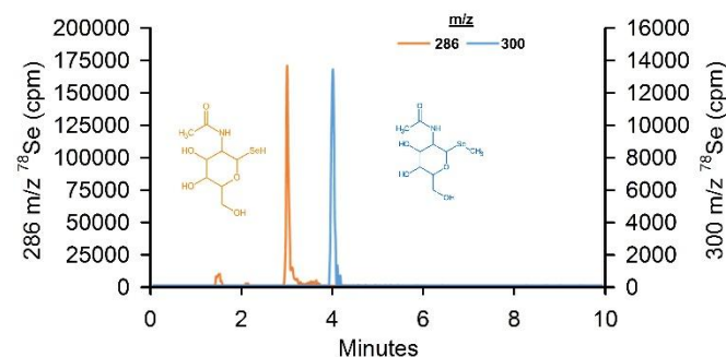
Fig. 4 RP HPLC-ICP-MS chromatogram of Se species in the high molecular weight water-soluble fraction after DTT reduction. Water extract of lyophilized liver from turkeys fed 5 µg Se/g after removal of the low MW Se species, reduced with DTT, and analysed by RP HPLC - ICPMS. Shown is the resulting chromatogram showing the m/z 286 Se species, SeGalNac (orange), and the m/z 300 Se species, methyl-SeGalNac (blue). Note the different 78 Se scales.
