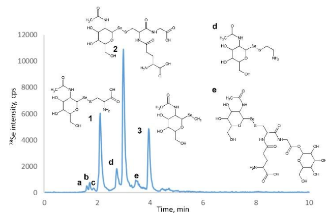
Fig. 3 Speciation of low-molecular weight (cutoff 3 kDa) water-soluble selenium in liver from turkey fed high Se (5 µg Se/g). Shown as a representative RP HPLC – ICP MS chromatogram. The Se species were identified by electrospray MS in a parallel experiment. 1, m/z 405; 2, m/z 591; 3, m/z 300. Minor selenospecies: a, b, c, not identified; d, m/z 361 (cysteinyl-SeGalNac); e, m/z 753 (glutathionyl-hexose-SeGalNac).
