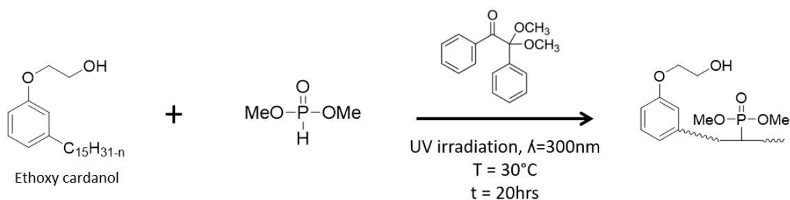
Scheme 3: Phosphorylation of ethoxy cardanol by UV irradiation radical reaction.
