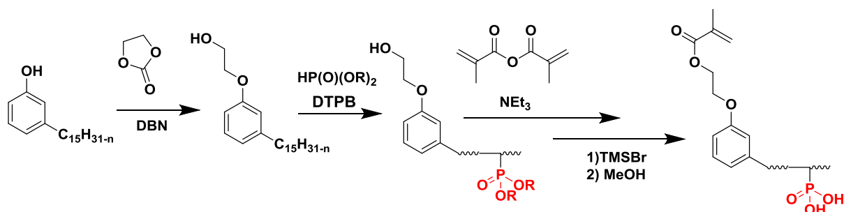
Scheme 1: General strategy of the synthesis of phosphonated cardanol methacrylate
