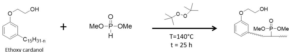
Scheme 2: Phosphorylation of ethoxy cardanol by thermal radical addition.
