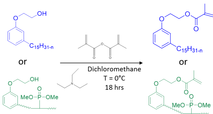
Scheme 4: Methacrylation of ethoxy cardanol and phosphonated ethoxy cardanol.
