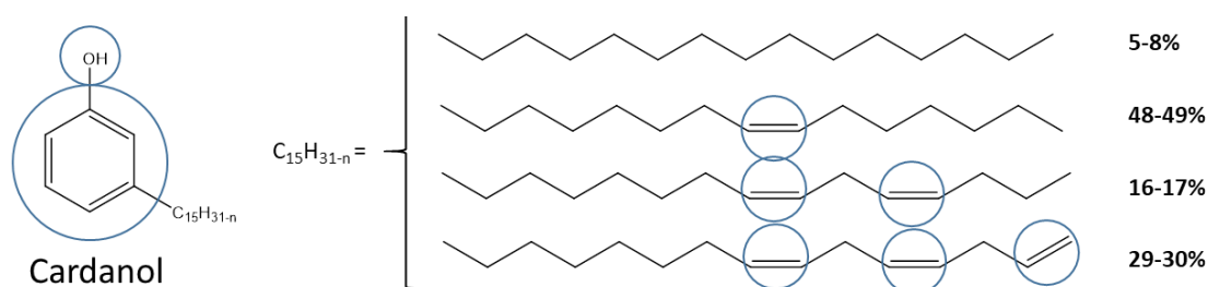
Figure 1 : Structure of cardanol
