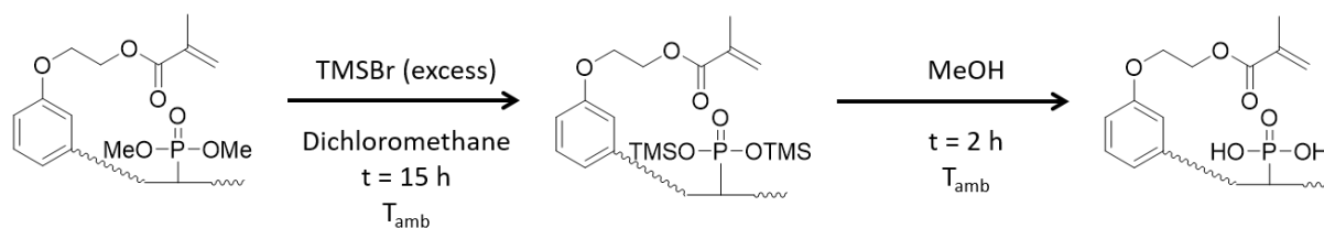
Scheme 5: Ester cleavage of phosphonate to phosphonic diacid using TMSBr in dichloromethane followed by methanolysis of the phosphorylated ethoxy cardanol methacrylate.
