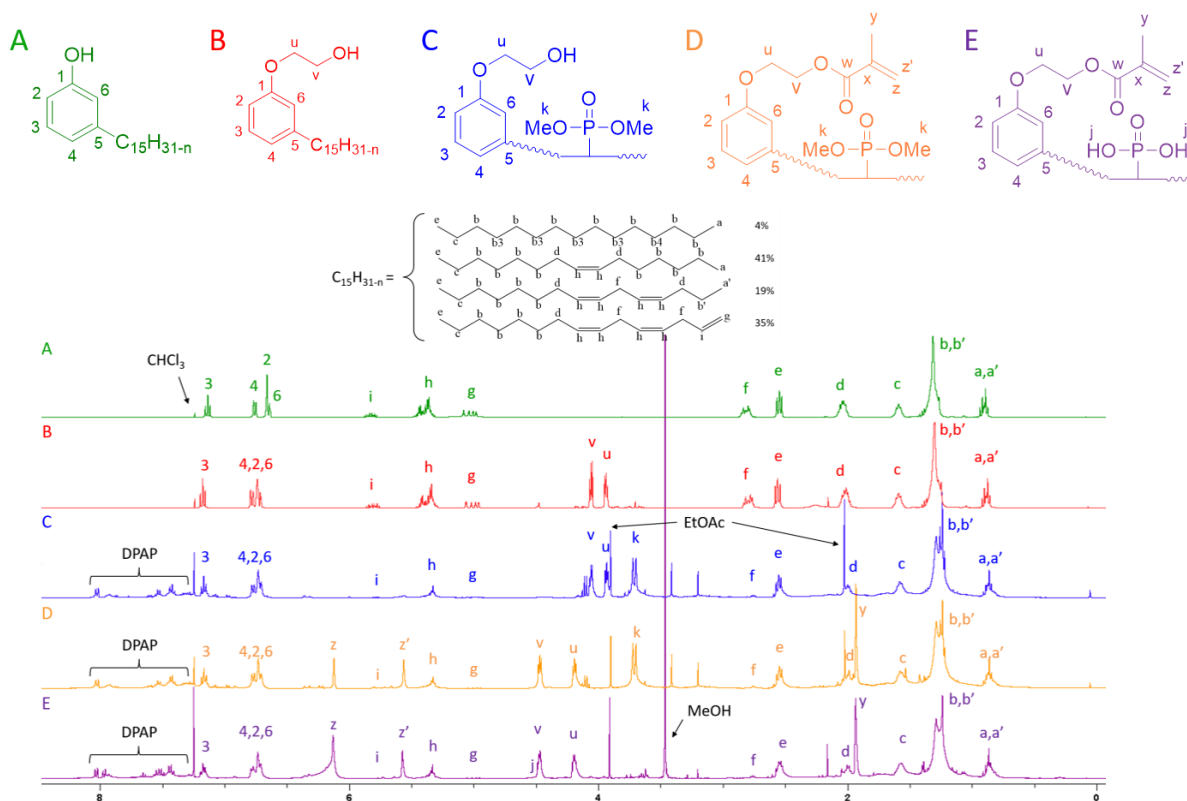
Figure 1: ^1\text{H} NMR spectra in \text{CDCl}_3 of . A: cardanol, B: ethoxy cardanol, C: phosphonated ethoxy cardanol via UV-mediated addition, D: phosphonated ethoxy cardanol methacrylate, E: phosphonic ethoxy cardanol methacrylate.
