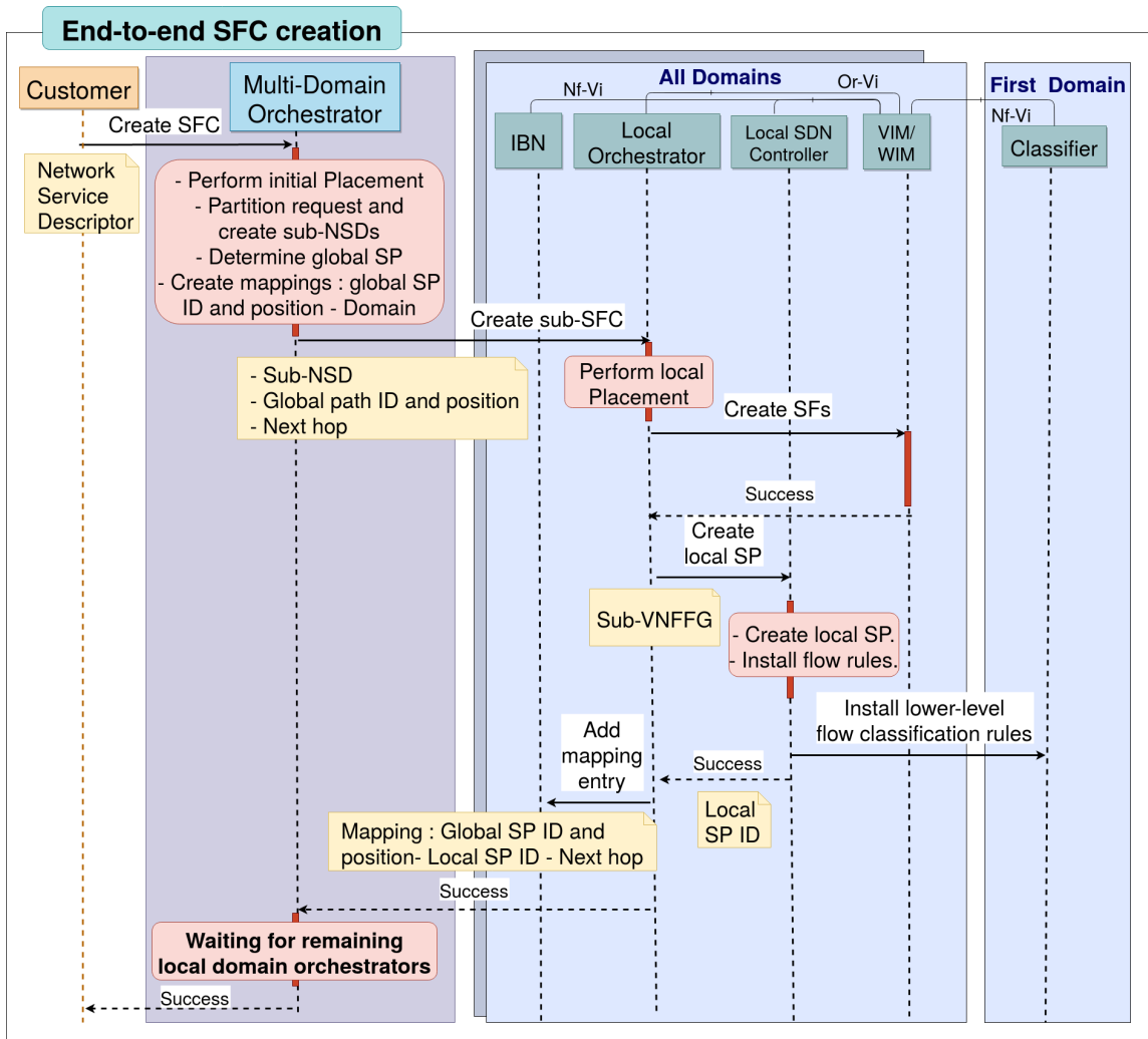
Figure 2: Multi-domain SFC instantiation workflow
