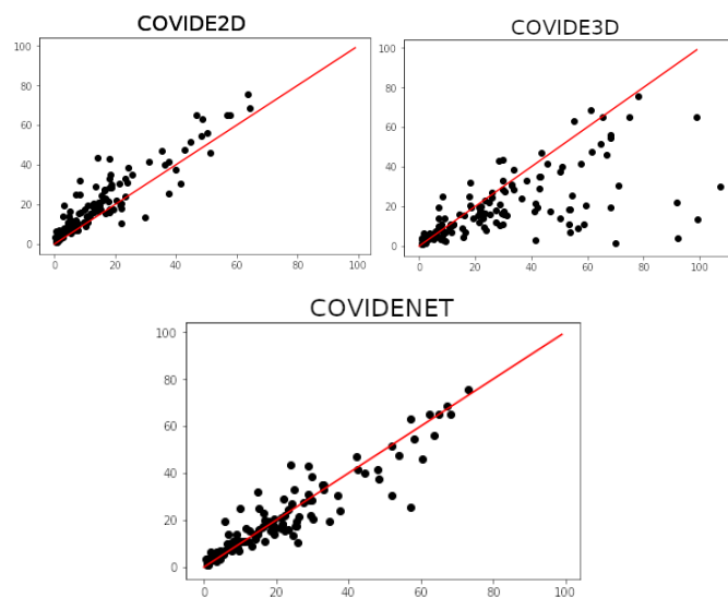
Fig. 5. Plots indicating the correlation between disease extent automatically measured and the average disease extent measured from CovidE2D, CovidE3D and CovidENet respectively and the manual segmentation. Disease extent is expressed as the percentage of lung affected by the disease. The red line shows a perfect correlation (Spearman R = 1 ). Spearman correlation coefficients are displayed for each comparison.
