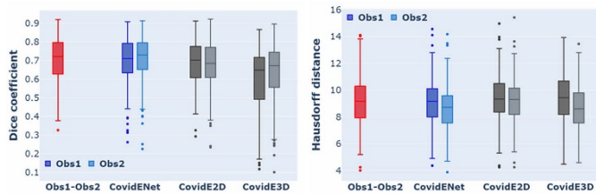
Fig. 4. Box-Plot in terms of DSC and HD between CovidENet and its individual components, Obs1 & Obs2. One can observe that CovidENet (blue) performs better and closer to Obs1-Obs2 (red) DSC and HD metrics than its individual components CovidE2D & CovidE3D.
