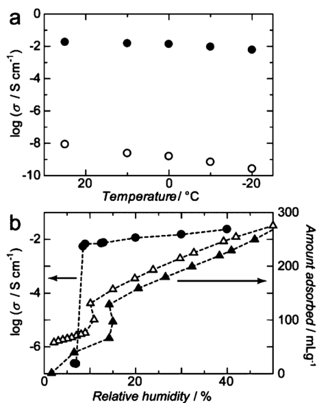
Fig. 31 (a) Arrhenius plots of ion conductivity for CaMOF- x H 2 O (open circles) and CaMOF-LiCl- x H 2 O (filled circles) at RH = 40%. (b) Humidity dependency of ion conductivity for CaMOF-LiCl- x H 2 O at 25 °C (filled circles). The H 2 O adsorption (filled triangles) and desorption (open triangles) isotherms of 1-LiCl at 25 °C. Reprinted with permission from ref. 172 .
