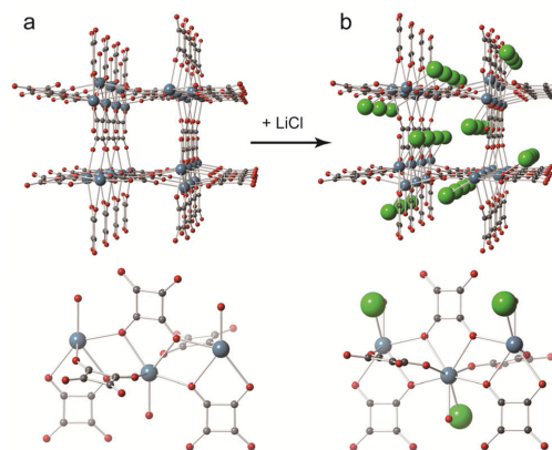
Fig. 30 Crystal structures: (a) CaMOF · xH 2 O at 10 °C and (b) CaMOF-LiCl · xH 2 O at -50 °C along the c -axis (top) and the coordination environments around the Ca 2+ ions (bottom). Non-coordinating water molecules are omitted for the sake of clarity. Blue, gray, red, and green are Ca 2+ , carbon, oxygen, and chlorine respectively. For chlorine, one disordered position is displayed. Reprinted with permission from ref. 172 .
