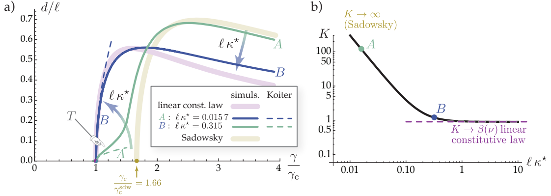
Figure 4.3. (a) Numerical solutions to the lateral-torsional buckling problem, obtained using AUTO-07p for \nu = 0.4 . The scaled lateral deflection d/\ell = |\mathbf{r}(\ell) \cdot \mathbf{e}_x|/\ell is plotted as a function of the dimensionless load parameter \gamma/\gamma_c . The thin curves are the predictions of the extensible ribbon model, for a thinner ribbon (A, \ell\kappa^* = 0.0157 ) and a thicker ribbon (B, \ell\kappa^* = 0.315 ). The dashed half-parabolas are Koiter’s weakly non-linear predictions from equation (4.5). For thin enough ribbons such as A, the initial buckling regime produces a tongue T in the bifurcation diagram. The thick, light brown curves are the predictions of the linearly elastic rod model and of Sadowsky’s inextensible ribbon model. (b) Log-log plot of the initial curvature K predicted by Koiter’s weakly post-buckling analysis, as a function of the parameter \ell\kappa^* .
