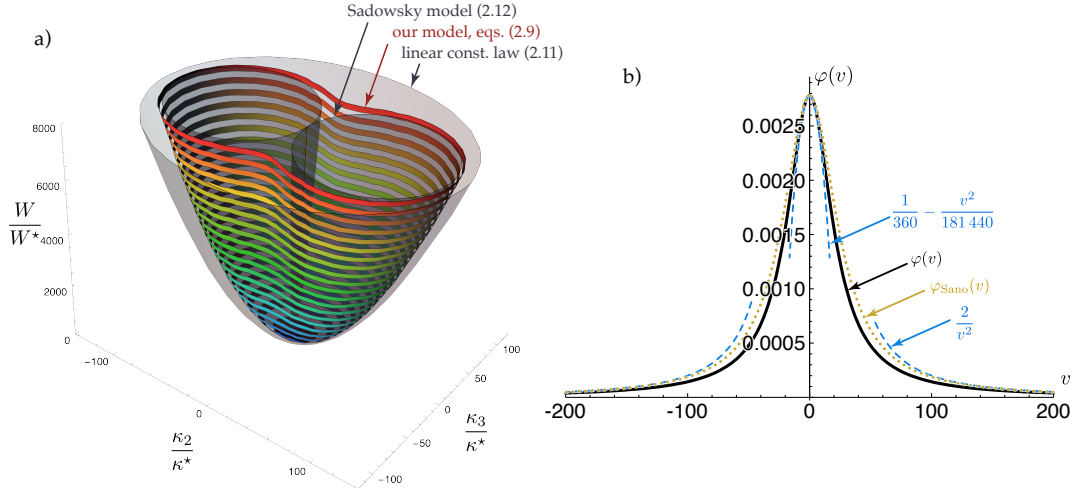
Figure 2.2. (a) Scaled strain energy W/W^* , as predicted by equation (2.9) for \nu = 0.4 , as a function of the scaled bending strain \bar{\kappa}_2 = \kappa_2/\kappa^* and of the scaled twisting strain \bar{\kappa}_3 = \kappa_3/\kappa^* . The strain energy of our equivalent rod model for the ribbon (colored surface) is well approximated by a quadratic strain energy (2.11) when both \kappa_2/\kappa^* and \kappa_3/\kappa^* are small (outer transparent paraboloid) and by Sadowsky energy (2.12) when \kappa_2/\kappa^* is large (double inner tube). (b) Graph of the function \varphi(v) defined in equation (2.8) (black solid curve) as well as its equivalents for small and large strain (blue dashed curves) and its approximation \varphi_{\text{Sano}}(v) from equation (3.6) (dotted orange curve).
