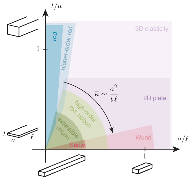
Figure 8.1. Tentative map showing the domains of validity of different theories for a prismatic elastic body having a rectangular cross-section with dimensions a \times t and length \ell , and experiencing finite rotations, \kappa = \mathcal{O}(1/\ell) : Kirchhoff theory (‘rod’), a typical higher-order rod theory, Sadowsky inextensible ribbon model (‘Sadw’), Wunderlich inextensible ribbon model (‘Wund’), the present extensible ribbon model, a typical high-order extensible ribbon model (to be derived in future work), a 2D plate model, and the 3D elasticity theory.
