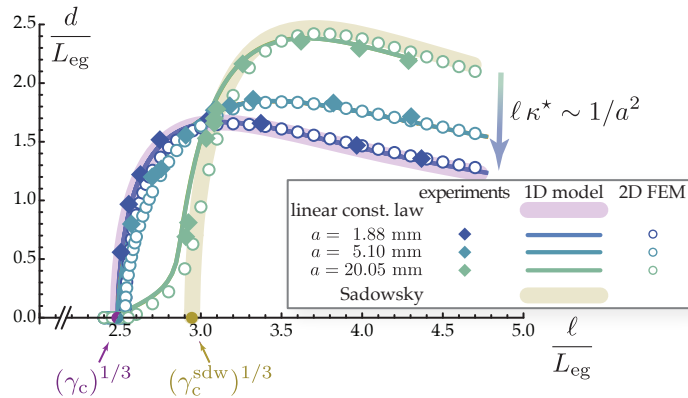
Figure 4.4. Comparison of the bifurcation diagrams for the lateral-torsional buckling of three ribbons having different widths, with thickness t = 0.0925 mm: experiments using a cellulose acetate sheet (filled diamonds), numerical simulations of the one-dimensional model using AUTO-07p (thin curves), and finite-element simulations of the Naghdi shell model (open disks). The simulations of both the one-dimensional rod model and of the two-dimensional shell model use a Poisson's ratio \nu = 0.4 , which is typical of the material used in the experiments. A single parameter, L_{\text{eg}} = 62.3 mm, has been adjusted.
