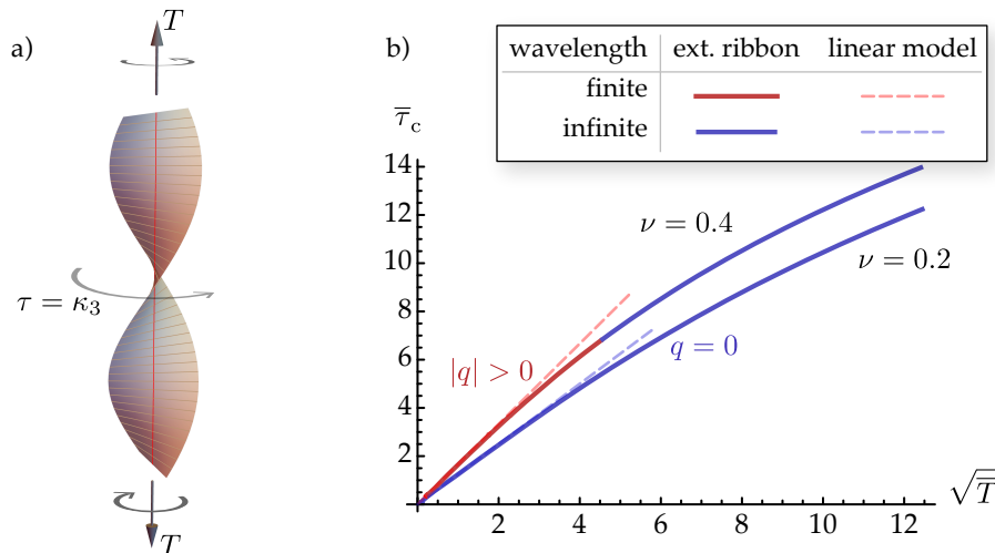
Figure 5.1. Linear bifurcation analysis of a twisted ribbon having infinite length. (a) Geometry. (b) Scaled first critical twisting strain \bar{\tau}_c = \tau_c / \kappa^* as a function of the square root of the scaled applied tension \bar{T} = T / W^* ; see equations (2.7) and (2.10) for a definition of the scales \kappa^* and W^* . The solid curves are the predictions of our ribbon model from equations (5.1–5.3); the dashed lines are the predictions of the small-tension approximation from equation (5.4). Note that the instability switches from finite-wavelength (red, |q| > 0 ) for larger values of \nu and for moderate applied tension, to infinite-wavelength (blue, q = 0 ) for smaller values of \nu or larger applied tension.
