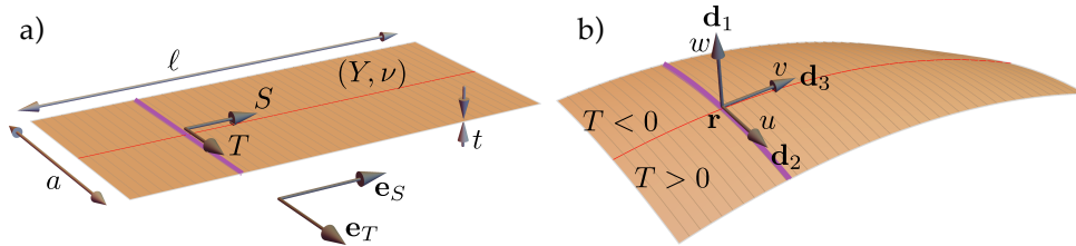
Figure 2.1. An elastic ribbon in (a) reference and (b) actual configurations. A particular cross-section with coordinate S is highlighted in purple color.
