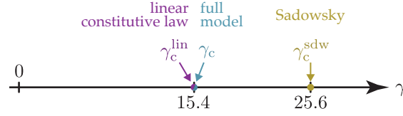
Figure 4.2. First critical buckling load for the lateral-torsional buckling, as predicted by the different models, for \nu = 0.4 , from equation (4.4). Note that the predictions from the extensible ribbon model (section 2) coincides with that from the linearly elastic model, and that Sadowsky’s model predicts a buckling load that is 66% larger for this particular value of \nu .
