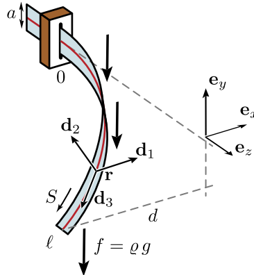
Figure 4.1. Lateral-torsional buckling of a ribbon: typical buckled configuration. The buckling amplitude is measured by the horizontal deflection d = |\mathbf{r}(\ell) \cdot \mathbf{e}_x| of the endpoint.
