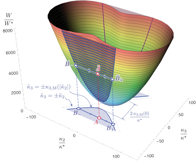
Figure 7.1. Convexified strain energy for \nu = 0.4 . The strain values that coexist across a discontinuity (Maxwell pairs) are denoted as (B_-, B_+) ; they are given by equation (7.3) or equations (7.5–7.6). When lifted onto the energy surface, they yield the points (\tilde{B}_-, \tilde{B}_+) that sit on the edge of the concave part of the energy surface: replacing this concave part by the surface swept by the segments joining \tilde{B}_- and \tilde{B}_+ (semi-transparent blue surface in the figure), one obtains the convexified energy surface. In the plane shown at the bottom, the blue shaded regions containing the point A corresponds to macroscopic strain values that give rise to a microscopic mixture of the phases B_- and B_+ .
