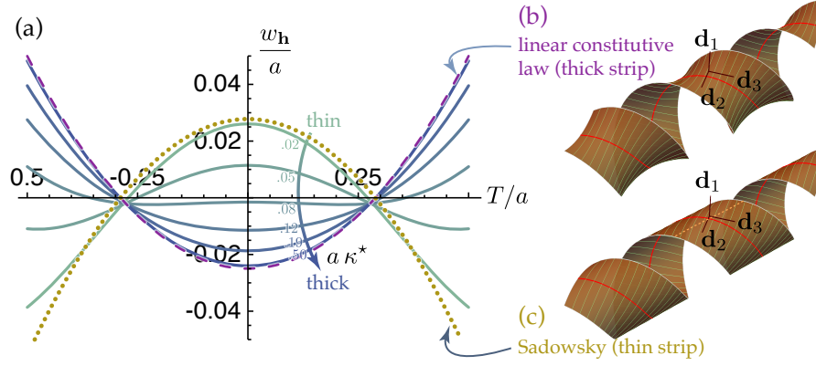
Figure 2.3. (a) Dependence of the deflection w_h(T) on the ribbon thickness t , for a helical solution. The scaled deflection w_h/a is plotted as a function of the scaled transverse coordinate T/a based on equation (2.13). The width a and the macroscopic strain \kappa_2 and \kappa_3 are held constant, with a\kappa_2 = -1.5 and a\kappa_3 = 1 ; Poisson's ratio is set to \nu = 0.4 . The various curves correspond to different values of the thickness t , with a\kappa^* \sim t/a ranging from 0.02 to 0.5. Darker curves correspond to thicker ribbons, and match the prediction of the linearly elastic model (3.3) (dashed curve) when a\kappa^* is large enough. Lighter curves correspond to thinner ribbons, and match the prediction of Sadowsky's theory (3.4) (dotted curve) when a\kappa^* is small enough. (b,c) Reconstruction of deformed ribbon in both limit cases: in the thick limit the ribbon displays anti-clastic curvature, as in the linearly elastic model; while in the thin limit the ribbon is developable, as in Sadowsky theory (see section 3 for details).
