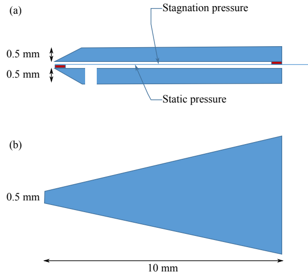
Figure 11. Schematic of the miniature Pitot sensor. (a) side view. (b) top view. The gap between the upper and lower parts is 20\ \mu\text{m} .
