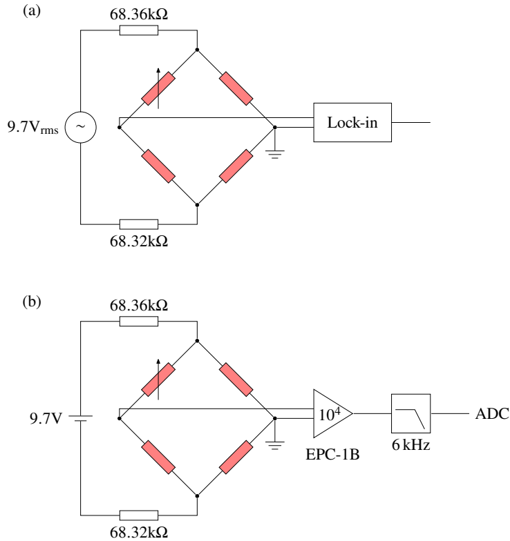
Figure 7. Electronic diagram for the cantilever measurements. The red resistor bridge is the Nichrome strain bridge micro-machined on the cantilever itself. Each resistor has nearly identical impedance of order 24 k \Omega . (a) Diagram for mean value measurements. The carrier wave frequency is 7 Hz, and the Lock-in amplifier time constant is 1 s. (b) Diagram for fluctuation measurements. In this configuration, frequencies below \sim 10 mHz are rejected by the EPC-1B low-noise amplifier.
