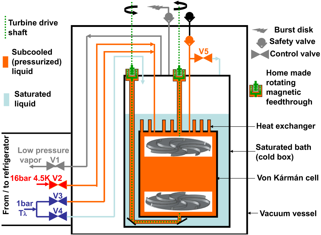
Figure 1. Schematic view of the SHREK experimental setup. The mean pressure of the flow is 3.0 bar.
