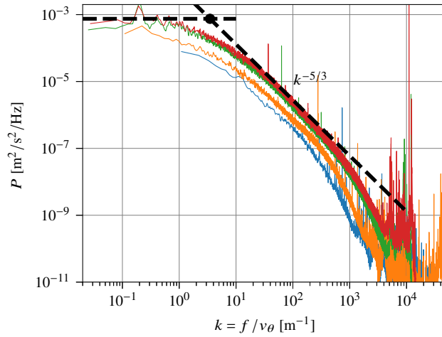
Figure 18. Velocity power spectra obtained in He I (2.3 K) in co-rotation with the hot-wire as a function of the wave number k . From bottom to top: \Omega = 0.19 \text{ rad/s} , \Omega = 0.50 \text{ rad/s} , \Omega = 2.20 \text{ rad/s} , \Omega = 3.77 \text{ rad/s} . The black dot is k_0 = 3.48 \text{ m}^{-1} at the intersection of the k^{-5/3} power law and the low wave number flat spectrum.
