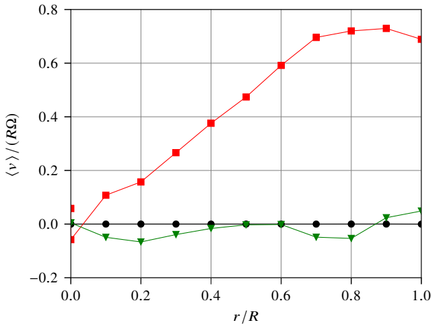
Figure 2. Velocity profiles obtained from Laser Doppler Velocimetry at mid-height in the SPHYNX Von Kármán cell. Red squares: azimuthal velocity; green triangles: vertical velocity; black circles: radial velocity derived from the continuity equation. The global Reynolds number is Re_g = 5 \times 10^5 .
