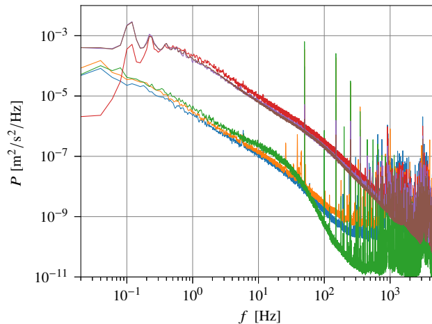
Figure 15. Velocity power spectra in He I and He II obtained with the cantilever with the Welch window adjusted so that 20 mHz is the lowest resolved frequency. From bottom to top: \Omega = 0.50 rad/s at 2.3 K (green), 2.0 K (orange), 1.58 K (blue); \Omega = 1.57 rad/s at 2.3 K (maroon), 1.98 K (violet), 1.58 K (red).
