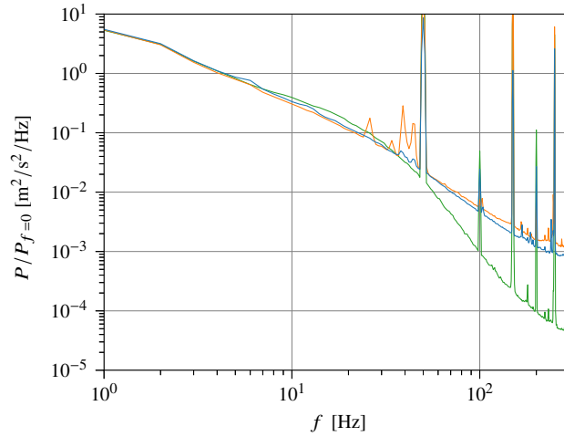
Figure 16. Cantilever-based velocity power spectra in He I and He II for \Omega = 0.50 rad/s with the Welch window adjusted so that 1 Hz is the lowest resolved frequency. The trend to saturation at high frequency is consistent with the expected noise floor from the electronics. Their level vary because of changes in sensor sensitivity. From bottom to top 2.3 K (green), 2.0 K (orange), 1.58 K (blue).
