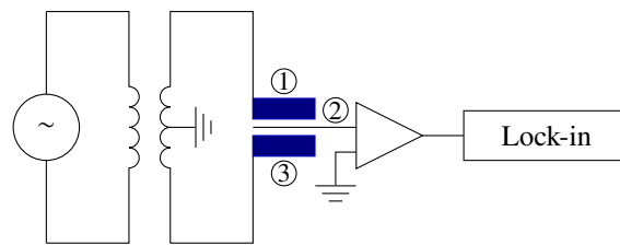
Figure 12. Electronic diagram of the capacitive readout for the miniature Pitot sensor. 1: Top electrode; 2: Membrane (mobile); 3: Bottom electrode.
