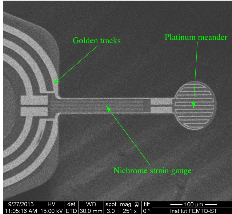
Figure 6. Scanning Electron Microscope picture of the cantilever anemometer.
