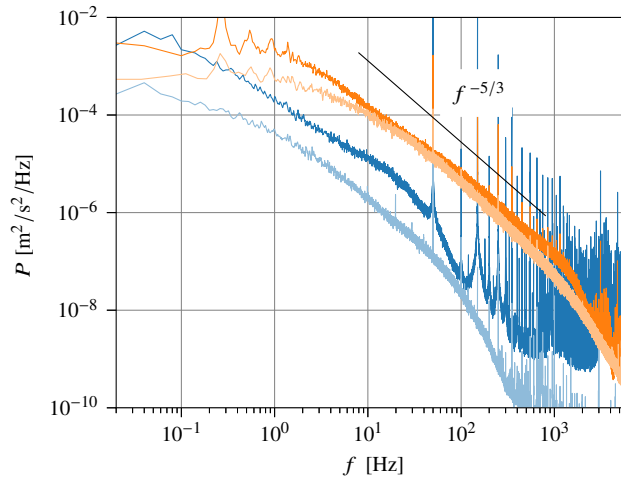
Figure 9. Turbulent velocity power spectra obtained with the cantilever in He I (2.3 K), using the quadratic calibration shown in Fig. 8 (dark lines), and the hot-wire (light lines) at angular velocities \Omega = 0.50 rad/s (bottom) and 3.77 rad/s (top). Black line shows the -5/3 slope.
