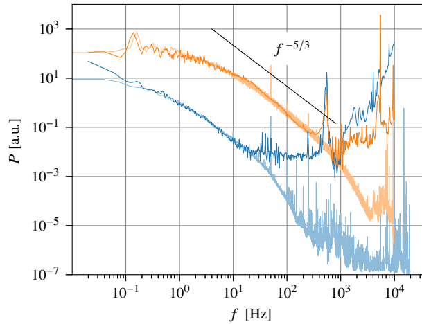
Figure 14. Power spectra obtained in He I ( T = 2.30 K) at \Omega = 0.31 rad/s (bottom), and \Omega = 2.20 rad/s (top), with the hot-wire signal (light color), and the miniature Pitot signal (dark color).
