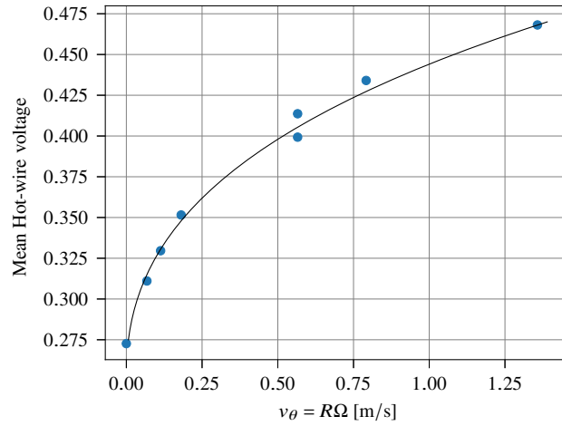
Figure 3. In-situ calibration of the hot-wire anemometer in He I. Solid line: King's law fit Eq. (3).
