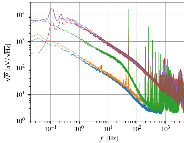
Figure 10. Power spectra of raw uncalibrated cantilever signal. From bottom to top: \Omega = 0.50 rad/s at 1.58 K (blue), 2.0 K (orange), 2.3 K (green); \Omega = 1.57 rad/s at 1.58 K (red), 1.98 K (violet), 2.3 K (maroon).
