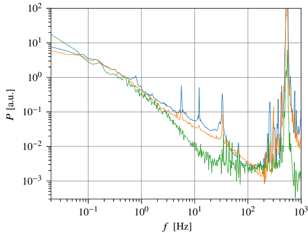
Figure 17. Velocity power spectra in He I and He II obtained with the miniature Pitot sensor for the angular velocity \Omega = 0.31 rad/s. From bottom to top: 2.3 K (green), 2.0 K (orange) and 1.58 K (blue).
