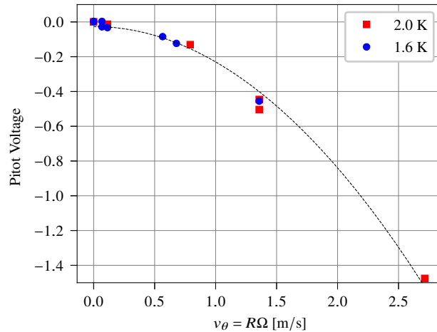
Figure 13. Mean voltage of the miniature Pitot sensor for several mean azimuthal velocities and temperatures in He II (1.6 K and 2.0 K). The dashed line is a quadratic fit.
