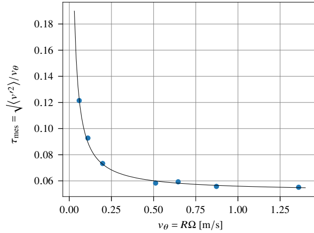
Figure 4. Measured turbulence intensity in He I, \tau_{\text{mes}} , computed from the hot-wire velocity signal, as a function of the azimuthal velocity. Solid line: fit using Eq. (7).
