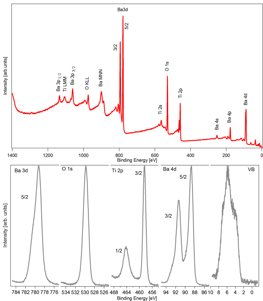
Figure 5. XPS survey (top) and core-levels and valence bands (VB) (bottom) of an undoped \text{BaTiO}_3 thin film recorded with monochromatized Al K_{\alpha} radiation.
