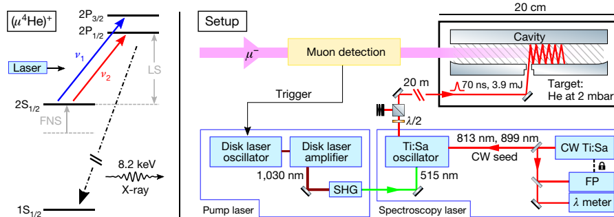
Fig. 1 | Energy-level scheme and experimental setup. Left: energy levels of interest in (\mu^4\text{He})^+ . We drive the 2S \rightarrow 2P transitions \nu_1 and \nu_2 (at wavelengths of 813 nm and 899 nm, respectively) and measure the 8.2-keV Lyman- \alpha X-ray from the subsequent decay to the 1S_{1/2} ground state. Indicated are the Lamb shift (LS) and the shift due to the finite nuclear size (FNS), which is proportional to r_\alpha^2 . Right: sketch of the experimental setup (not to scale). On the way to the He target, the muon is detected, thereby triggering the laser system. After the muon is stopped in 2 mbar of He gas at room temperature, (\mu^4\text{He})^+ is formed.
