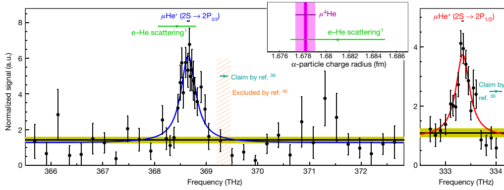
Fig. 2 | The measured transitions. The 2S \rightarrow 2P_{3/2} (left) and 2S \rightarrow 2P_{1/2} (right) resonances in (\mu^4\text{He})^+ fitted with a power-broadened Lorentzian line-shape at a fixed linewidth of 319 GHz (FWHM) given by the 2P lifetime. The black data points show the laser-induced events (number of X-rays in time coincidence with the laser light), normalized to the prompt events (number of X-rays from the cascade on formation of (\mu^4\text{He})^+ ). The horizontal band shows the background levels (with 1\sigma uncertainty) obtained from measured data where
