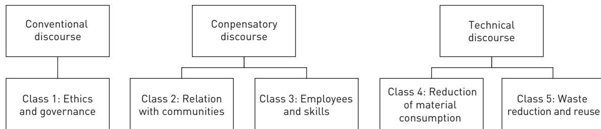
GRAPH 1 Class distribution
