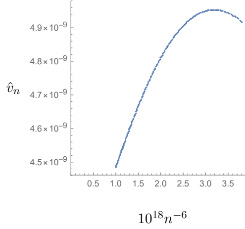
(b) Plot of \hat{v}_n = v_n - 166.95208957 vs. 10^{18}n^{-6} , where v_n approximates the constant term \gamma_r of relaxed trees.
