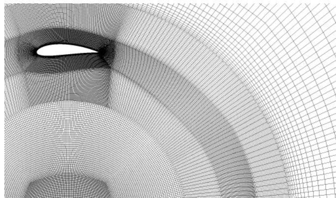
Figure 2: Close view of the mesh in the rotor region.
