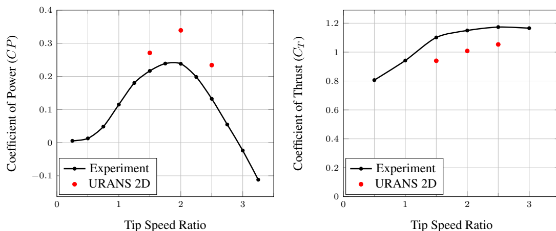
Figure 4: Comparison of measured and simulated coefficients of power (left) and coefficients of thrust (right).
