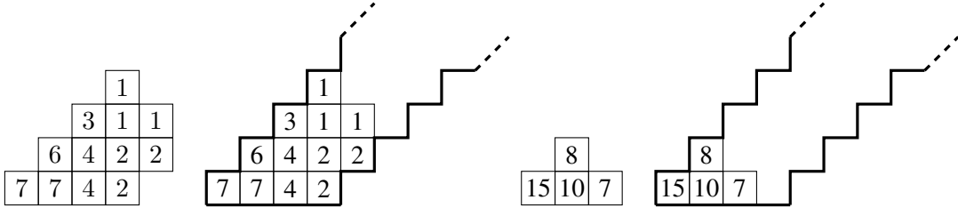
Figure 1: Two instances of banded plane partition of size 40 and width 4 (with and without the outer banded staircase).
