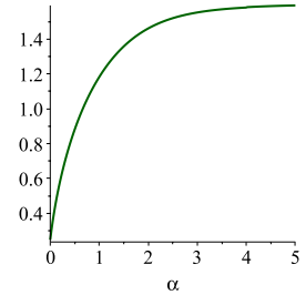
Figure 3: A plot of the increasing function G(\alpha) .
