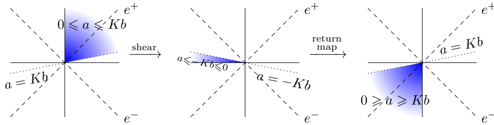
Figure 4.4. The cones in the proof of Proposition 4.3
