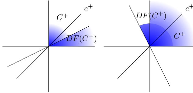
Figure 4.3. Action of a positive and negative twist (shear) on the first quadrant
