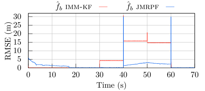
(b) RMSE barometer fault estimate.
