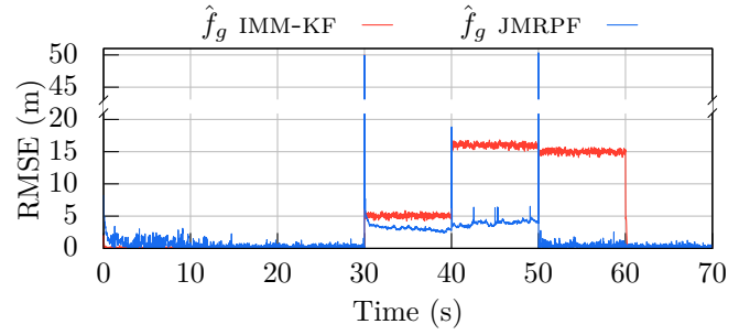
(a) RMSE GNSS fault estimate.
