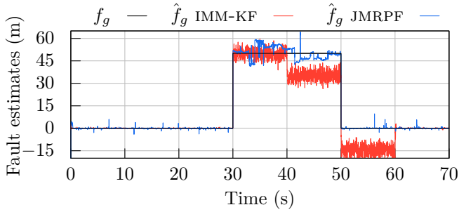
(a) GNSS fault estimates
