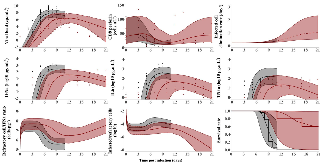
Figure 5 Model predictions (median and 95% prediction interval) for the compartments of the integrated model given in Figure 3c in animals left untreated (black) or treated with favipiravir 180 mg/kg BID. 69 The dots are the individual data in each compartment. Reproduced from ref. 69.
