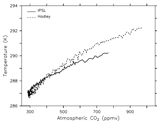
Fig. 2. Climate sensitivity (surface warming as a function of atmospheric \text{CO}_2 ) for IPSL (solid line) and Hadley (dashed line) coupled models.
