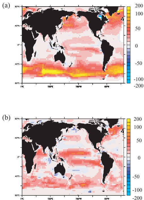
Fig. 4. Geochemical oceanic CO 2 uptake ( \text{gC m}^{-2} \text{yr}^{-1} ) at 700 ppmv for (a) the IPSL model and (b) the Hadley model uncoupled runs.
