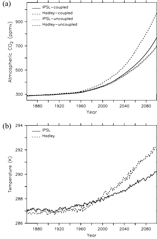
Fig. 1. Calculated atmospheric CO 2 and (b) surface temperature for the IPSL (solid line) and Hadley (dashed line) coupled runs. Atmospheric CO 2 obtained in the Hadley and IPSL uncoupled runs are also shown in (a).
