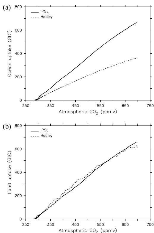
Fig. 3. IPSL (solid line) and Hadley (dashed line) carbon cycle models sensitivity to atmospheric \text{CO}_2 : (a) the oceanic uptake as a function of atmospheric \text{CO}_2 ; (b) the same for the land.
