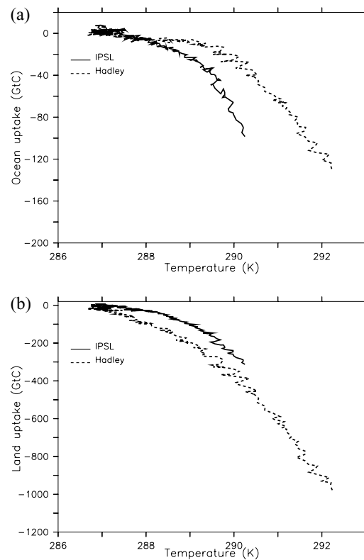
Fig. 5. Sensitivity of the IPSL (solid line) and Hadley (dashed line) carbon cycle models to climate change alone. (a) The change in oceanic uptake due to change in climate as a function of surface temperature; (b) the same for the land. As explained in the text, the fluxes have been corrected for the indirect climate effect through enhanced atmospheric CO 2 (see Fig. 1).
