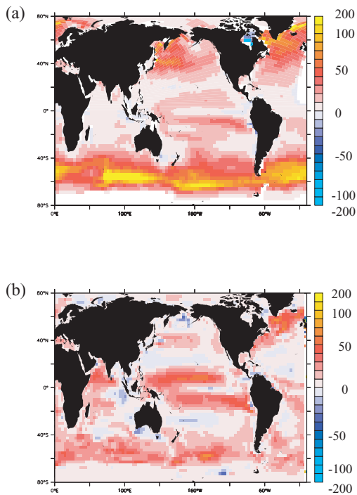
Fig. 4. Geochemical oceanic CO 2 uptake ( \text{gC m}^{-2} \text{yr}^{-1} ) at 700 ppmv for (a) the IPSL model and (b) the Hadley model uncoupled runs.
