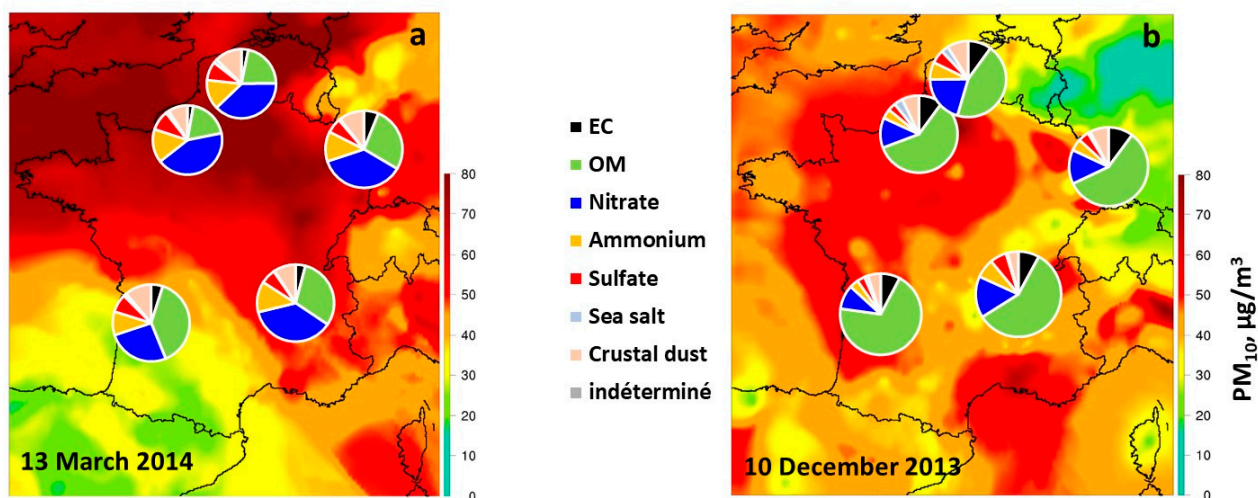
Figure 8. Examples of daily PM_{10} chemical composition observed for five urban stations (Lens, Rouen, Strasbourg, Lyon, and Bordeaux) during two different types of pollution episodes, along with PM_{10} concentration mapped using the Prev’Air modeling system ( http://www2.prevoir.org ) analyzed with in situ PM_{10} measurements. (a) 13 March 2014, (b) 10 December 2013
