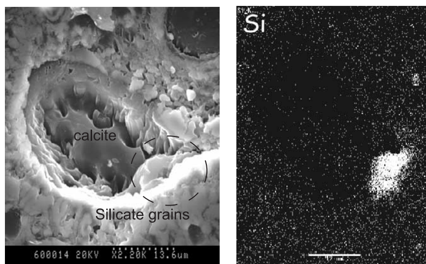
Figure 4. Example of a SEM X-ray map of a spot previously excavated by ion microprobe in the calcite part of a Globigerinoides test. Silica is also shown for the same spot and highlights the presence of micron-sized silicate grains, also rich in aluminum (not shown here), clearly incorporated within the calcite matrix. No grain is found in the pores located at depth and exposed by the sputtering. Scale bars are 12 \mu\text{m} .
