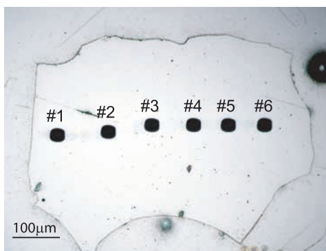
Figure 1. In situ \delta^7\text{Li} analyses performed in a single grain of CAL-HTP calcite standard. The corresponding spots are displayed on the picture underneath.
