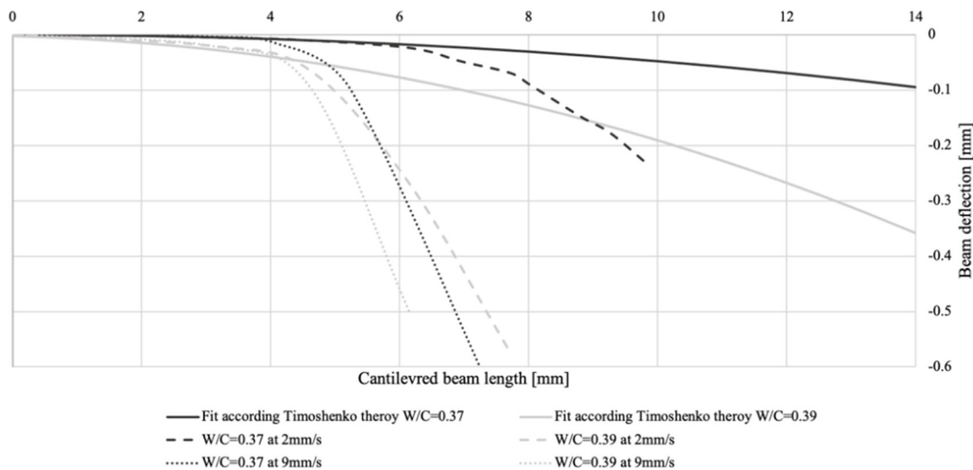
Figure 2. Tip deflection versus extruded specimen length. Comparison between experimental results and the Timoshenko beam theory for a material without CE
