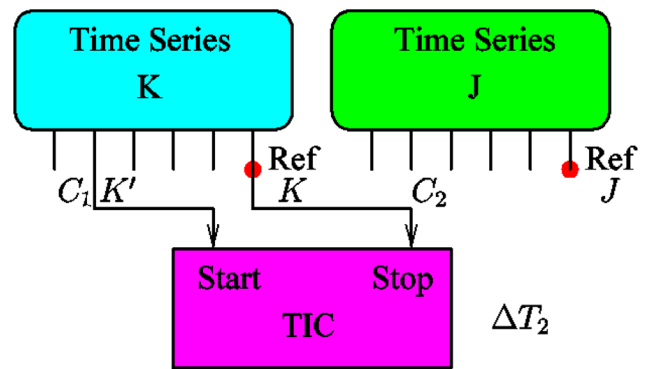
Figure 2. Illustration of the differential measurement technique called pivot. Cable C1 is connected to the pivot, while cable C2 is successively connected to the reference point of time series J and K . The difference between the measurements \Delta T_1 and \Delta T_2 provides the time difference between the two time series. Some uncertainties introduced by the TIC are mitigated, because they are common to both measurements, and no prior knowledge of the cables delays is needed.
