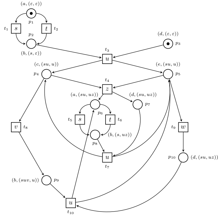
Figure 12: The spreading of the net in Figure 11
