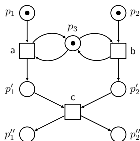
Figure 9: A multi-clock net with three components where the order of execution may play a rôle
