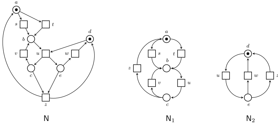
Figure 11: A multi clock net and its component
