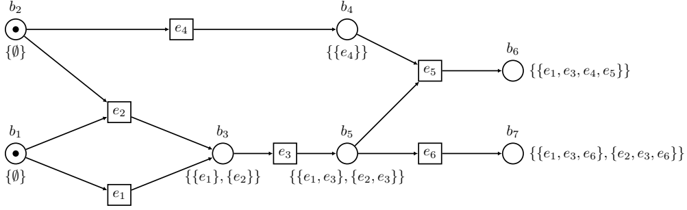
Figure 4: An unravel net
