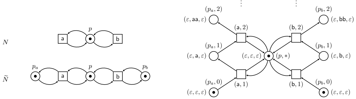
Figure 6: A multi-clock net with three components and its 1-unfolding
