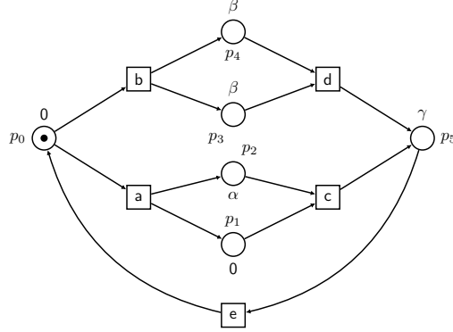
Figure 1: A spread net
