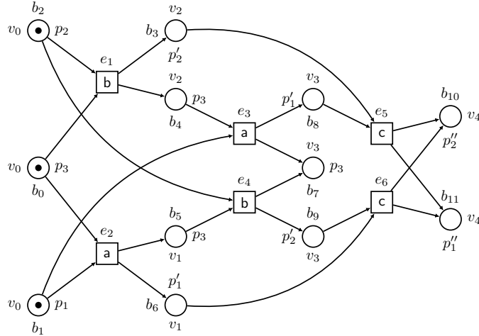
Figure 16: The spreading of the net in Figure 9 with respect to the domain induced by the automata for the local prefixes
