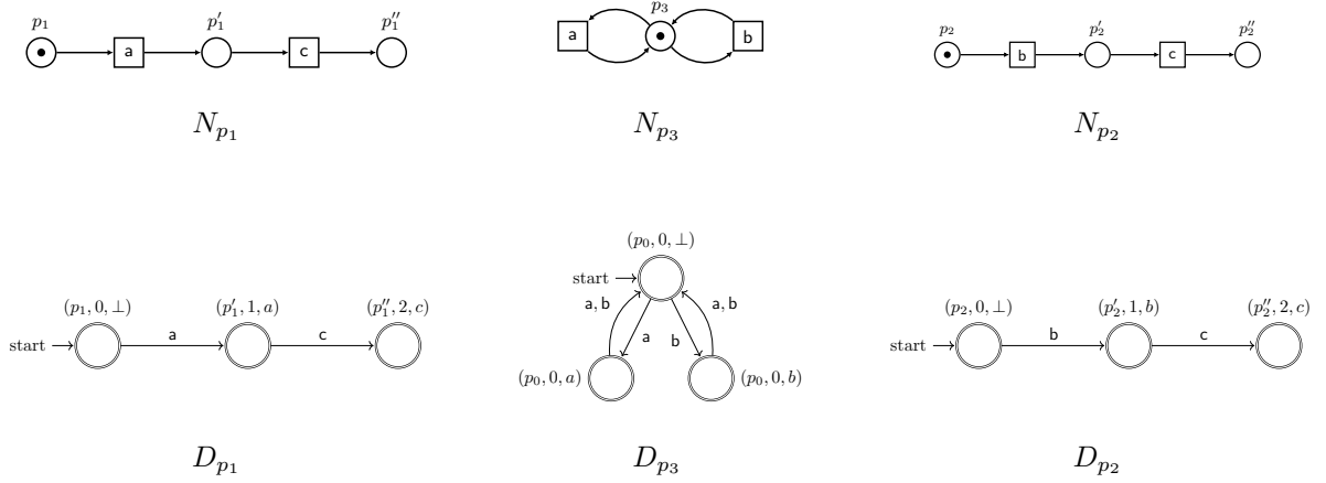
Figure 15: The three components of the multi-clock net in Figure 9 and the finite state automata associated to each of them.
