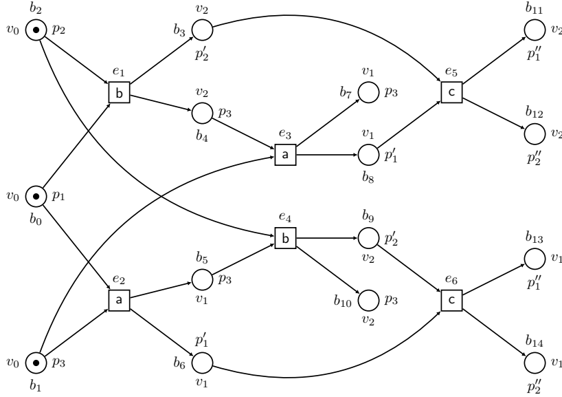
Figure 13: The spreading on the net in Figure 9 with the respect to the domain in Example 7.7
