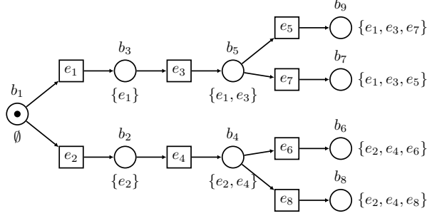
Figure 3: an occurrence net annotated on the information domain formed by subsets of events
