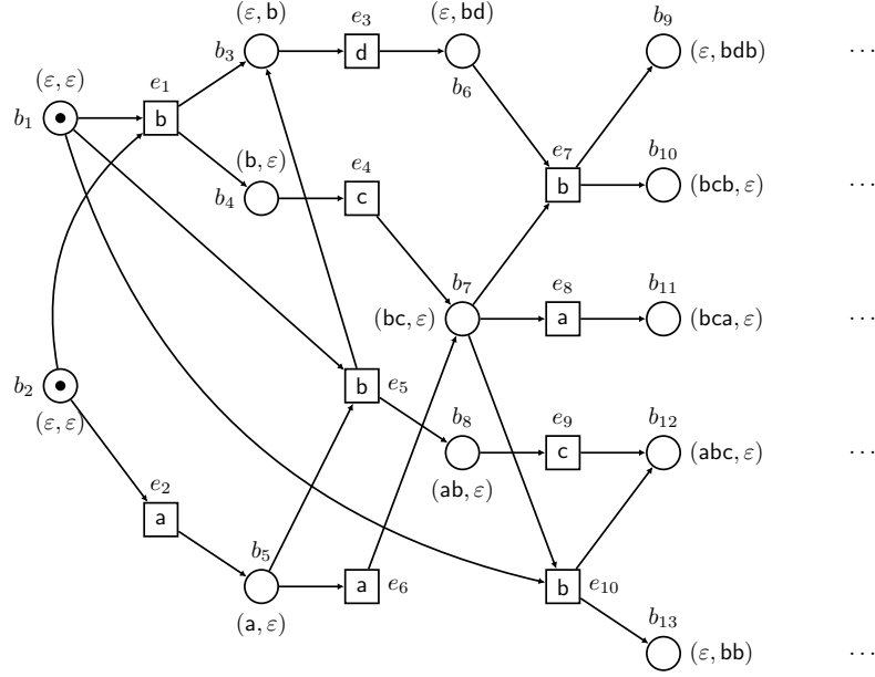
Figure 8: The spread net obtained by the initial part of the trellis process of Figure 5
