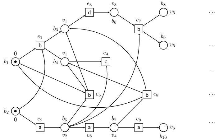
Figure 17: The initial part of the merged process of the net in Figure 5
