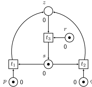
Figure 2: An 1-occurrence net annotated with an information mapping on \mathcal{D}_\perp
