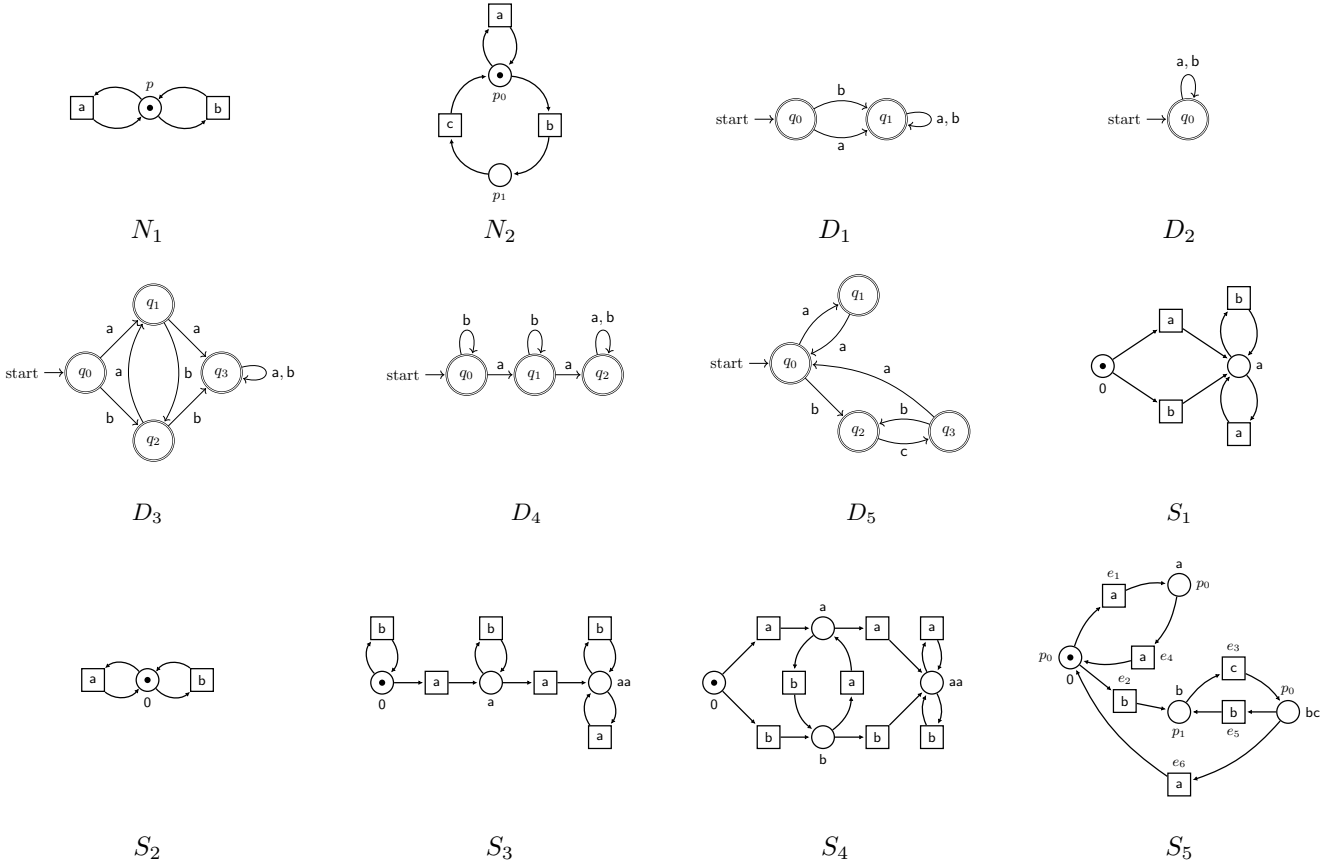
Figure 14: Two net automata N_1 and N_2 , five finite state automata for equivalence relations on words over \{a, b\} ( D_1, D_2, D_3 and D_4 ), a finite state automaton for an equivalence relation on words in \{a, b, c\} ( D_5 ), the spreading S_i of N_1 with respect to the domains D_i , 1 \leq i \leq 4 and the spreading S_5 of N_2 with respect to the domain D_5
