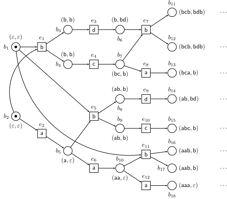
Figure 7: The spread net obtained by the initial part of the branching process of Figure 5
