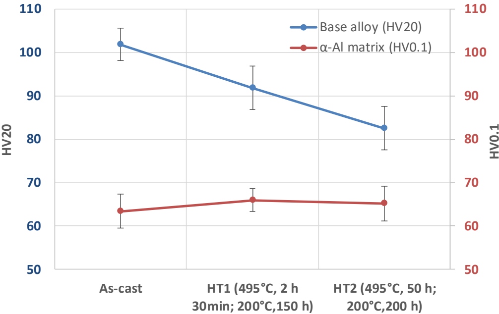
Figure 2 : Hardness as a function of various heat treatment conditions for base alloy and α-Al matrix
