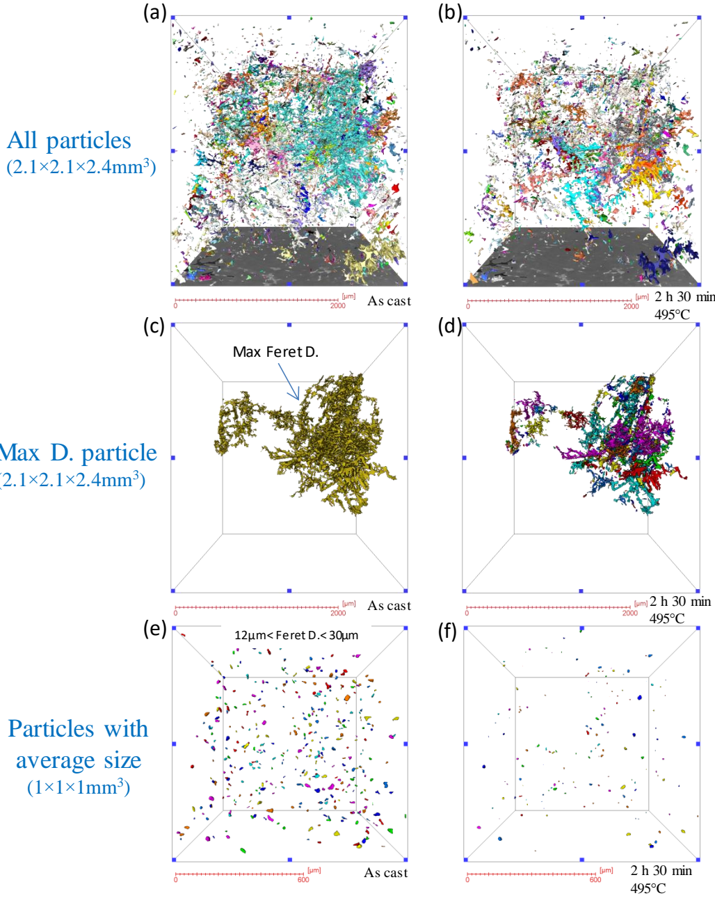
Figure 7: 3D rendering of the Al 2 Cu phase, from top to bottom: all the particles and the largest particle in the same 2.1×2.1×2.4 mm 3 region, particles having a Feret diameter between 12 to 30µm in a sub-volume (1×1×1 mm 3 ) at: (a, c and e) as-cast condition and (b, d and f) after 2 h 30 min at 495 °C for specimen HT1
