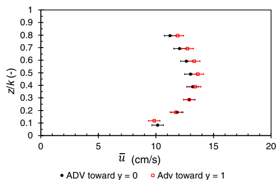
Fig. 6 Vertical profile of the longitudinal time-averaged velocity \bar{u} at x = 12 m and y/(L/2) = 6 , towards the glass sidewall located at y = 0 , or towards the plexiglass sidewall positioned at y = 1 ; after taking into account the correction alignment angle of the probe (Table 4) for the flow H/k = 0.93 .
