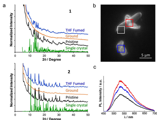
Figure 3. a) PXR D patterns of the pristine, ground and THF-fumed powders, and comparison with the data derived from X-ray diffraction analysis of a single crystal of 1 (top) and 2 (bottom). b) Fluorescence microscopy image of microcrystals of 2 . \lambda_{\text{ex}} = 400 nm. c) The corresponding emission spectra. The colours of the spectra refer to the zone where the emission signal was taken, except for the white zone, which gives the black spectrum.
