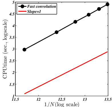
Figure 2: Computational time for the evaluation of the convolution by the fast algorithm vs N (for M = 160 ).
