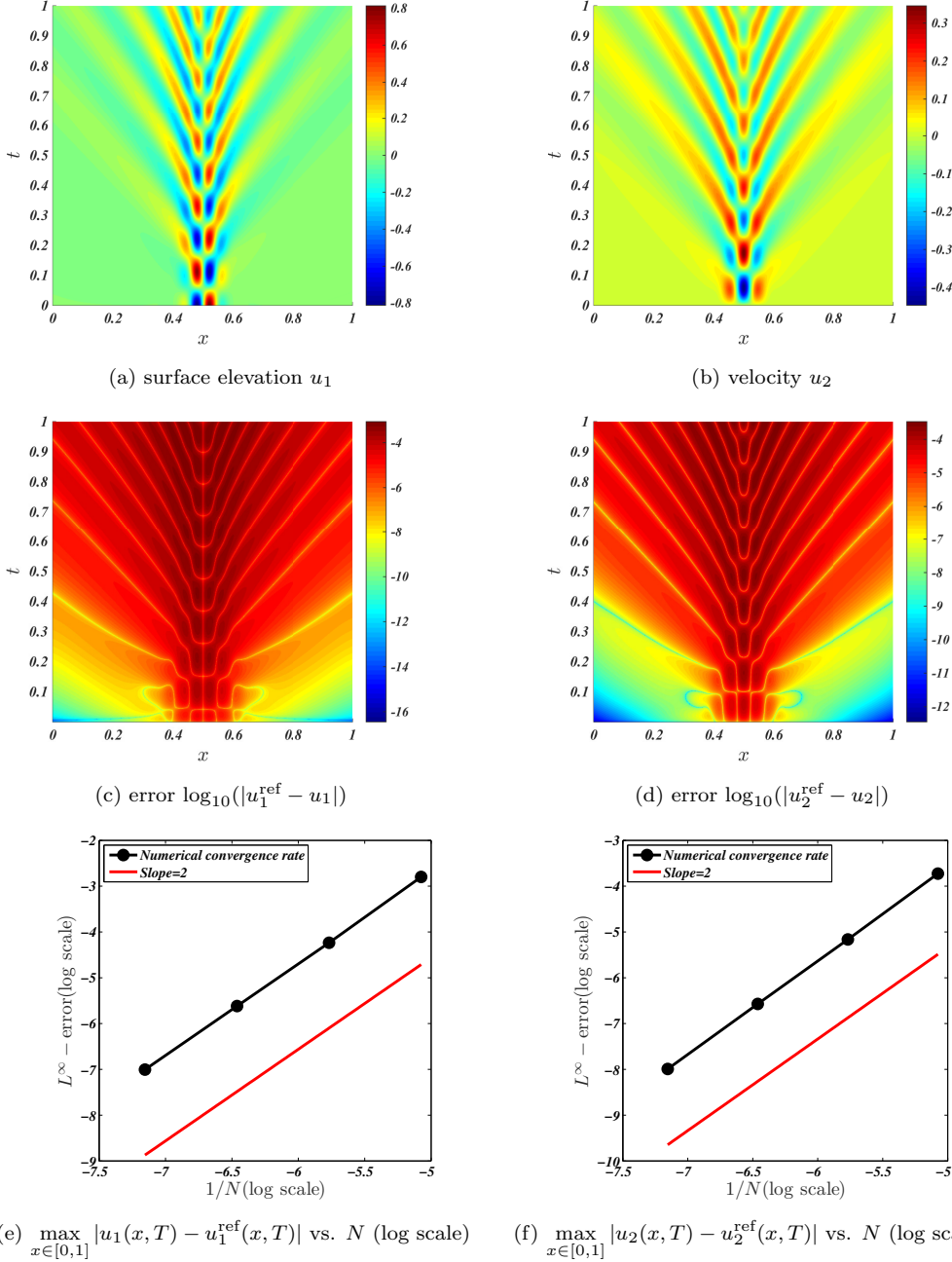
Figure 1: Illustration of the accuracy of the scheme for both the boundary reflection and the convergence rate.
