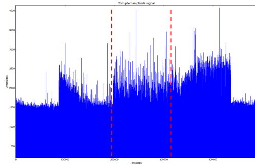
Fig. 7. Corrupted amplitude signal in the first scenario; the intruder is active in the time slot between the dashed lines.
