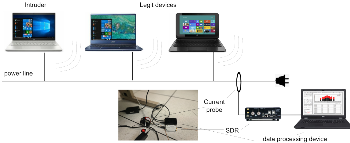
Fig. 1. Block diagram of the proposed method: the network is made of legit devices and an intruder. All generate EM emanations that couple onto the power lines. IDrISS captures the EM signal with a current probe and SDR system that sends the raw IQ data to a processing data device.
