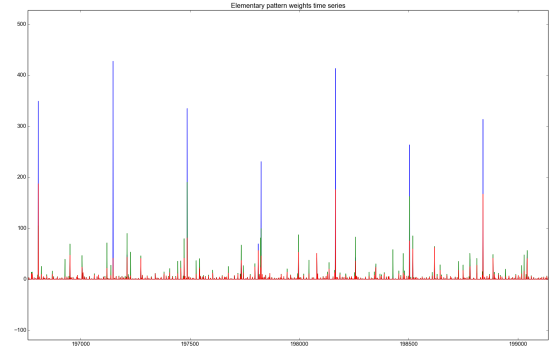
Fig. 6. Sparse vector-valued amplitude signal representation. Each color corresponds to one coordinate of the vector value at each time
