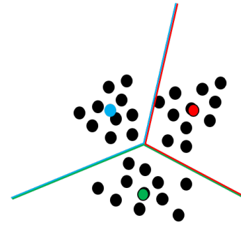
Fig. 5. Partitioning.
