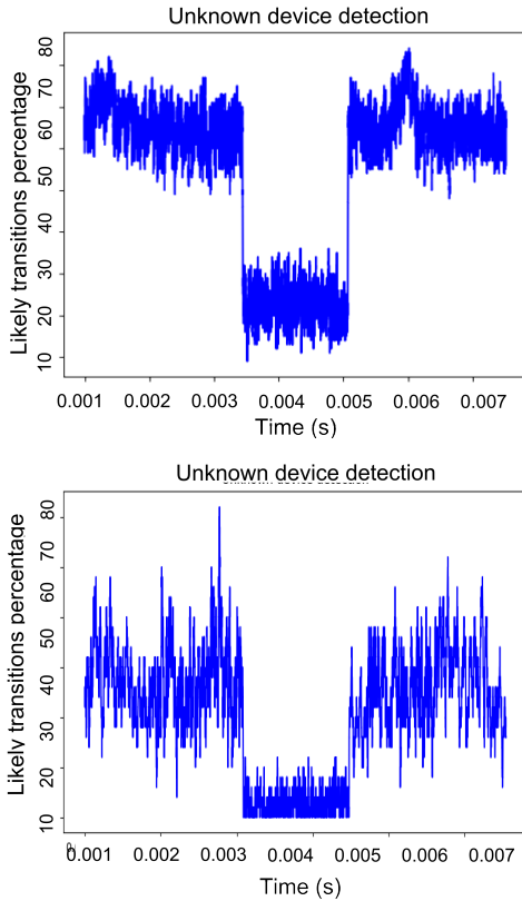
Fig. 9. Intrusion detection in the first scenario on the top and the second scenario on the bottom. The activation of the unknown equipment causes a detectable rupture thanks to the learned sequential model.
