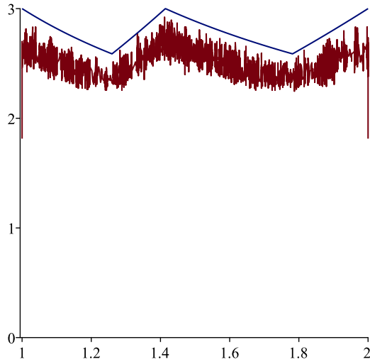
Fig. 6: The error bound for the computation of ax^3 as (a \cdot x) \cdot (x \cdot x) , in multiples of u and as a function of a \in [1, 2) , along with the largest actually obtained values for p = 16 .
