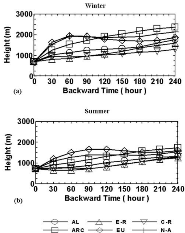
Figure 10. Average height above the ground as a function of time back for the 6 clusters for the 10 days back trajectories for (a) winter and (b) summer.
