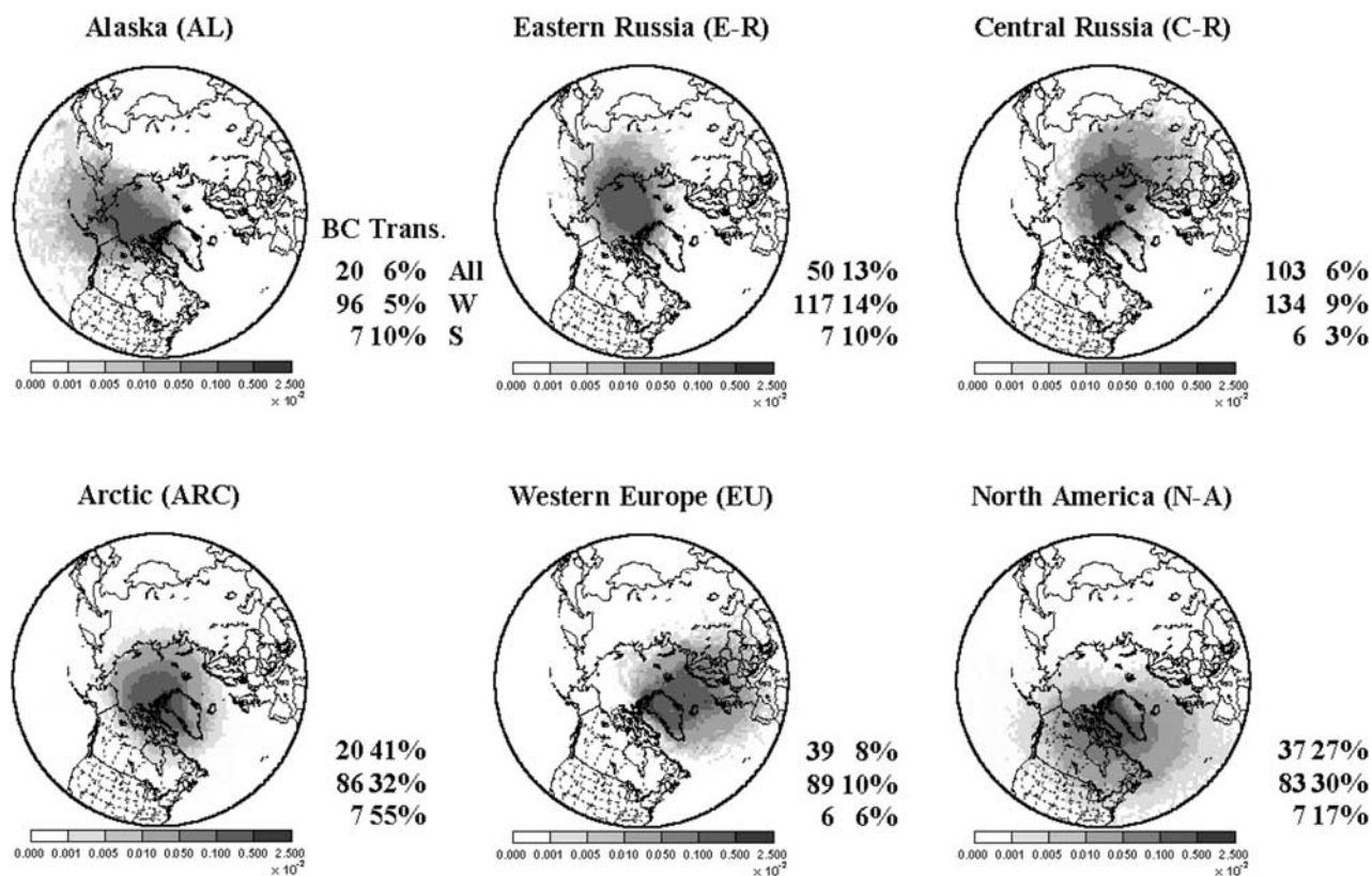
Figure 5. Sector analysis showing the probability density for 10-day back trajectories between 1989 and 2001 at Alert. Also given are the median BC concentrations ( \text{ng m}^{-3} ) for all year, winter, and summer for the sectors with the frequency of the transport from each sector.
