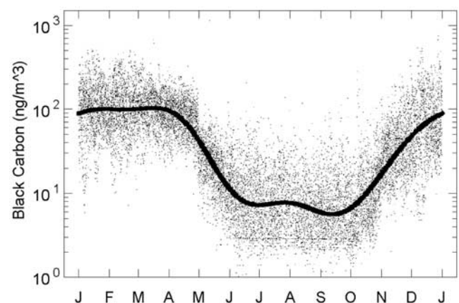
Figure 4. Seasonality in the corrected black carbon measurements for the data from 1989 to 2002.
