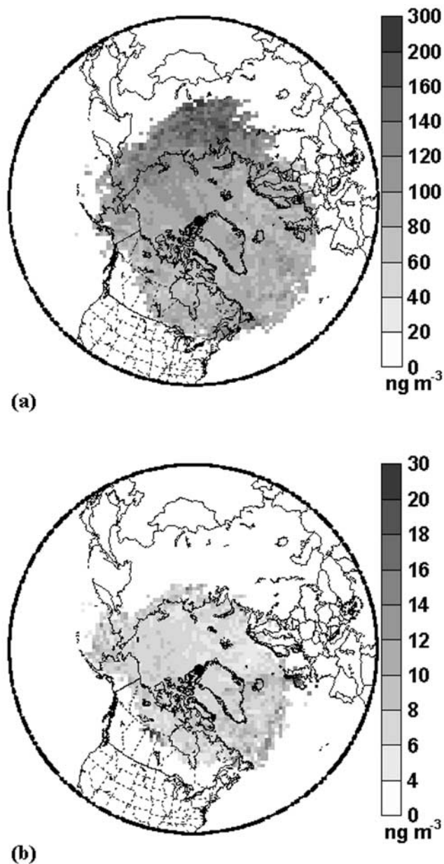
Figure 7. Upwind areas identified by trajectories for which BC measurements at Alert are high and low from 1989 to 2001 as generated by the Seibert et al. [1994] analysis for (a) winter (January to April) and (b) summer (June to September). For details, see text. Note the difference in scales between the two plots.
