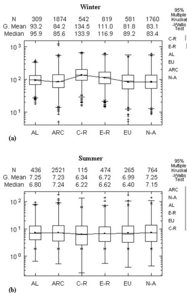
Figure 6. Distribution of 6-hourly mean BC concentrations associated with the back trajectories in the 6 clusters for the (a) winter and (b) summer showing the median, 25th percentile, and 75th percentile.
