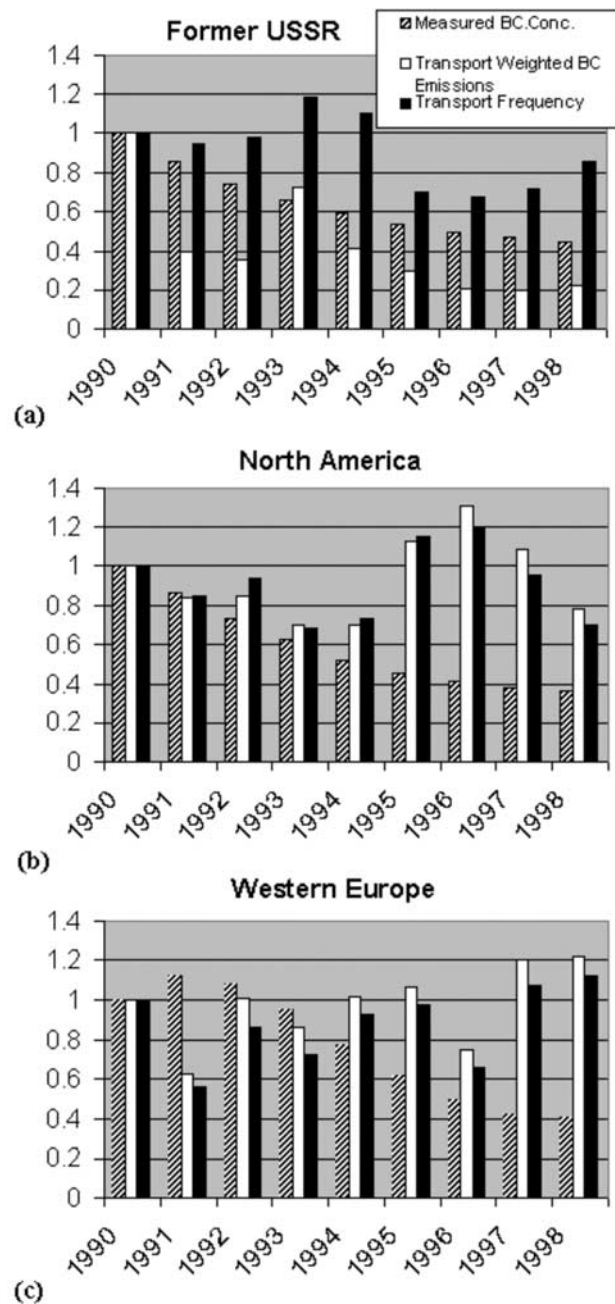
Figure 9. Changes relative to 1990 of BC air concentration geometric means, BC emissions, and transport frequency to Alert from (a) the former USSR, (b) North American, and (c) western European sectors.
