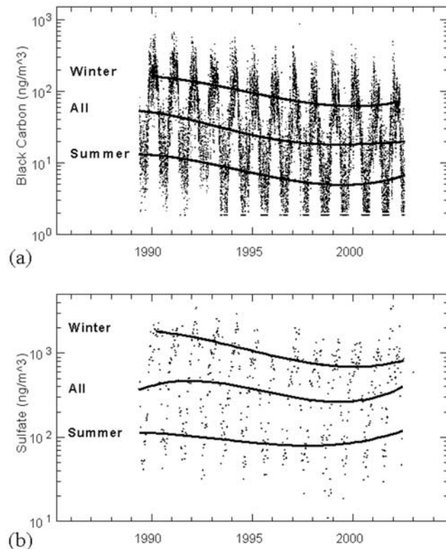
Figure 3. Times series of (a) corrected black carbon concentrations (on a logarithmic scale) and (b) sulfate concentrations from 1989 to 2002 at Alert showing a downward trend in the measurements.
