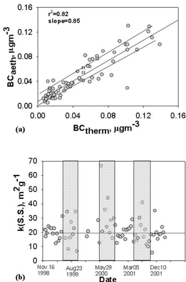
Figure 2. Relationship between (a) BC obtained from thermal versus optical technique showing a regression line and 1\sigma confidence limits and (b) the correction applied to the specific attenuation coefficient. The mean values for the site-specific attenuation were used to convert the light absorption measurements for the summer (highlighted) and winter.
