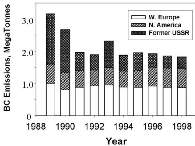
Figure 8. Average annual BC emissions for 1989–1998 for western Europe, North America, and the former USSR as computed by Cooke et al. 's [1999] method.
