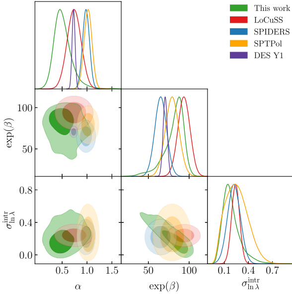
Figure 6. Identical MCMC-fitting results as in Fig. 3, but with the inclusion of the scaling relation results from the literature, rescaled at M_{200c} = 10^{14.81} M_{\odot} and z = 0.5 . Contours indicate the statistical 1\sigma (68 per cent) and 2\sigma (95 per cent) credible regions.
